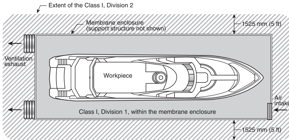
PLAN VIEW
