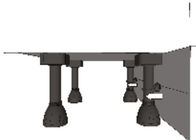
5 Screw the plinth clip back plate central to the markings made in the last step. Then slide the plinth Clips onto the back plates. Finally offer the plinth with the clips into place and slide the clips onto The back plates to line up with the legs before pushing the plinth into place allowing the clips to spring around the legs.
