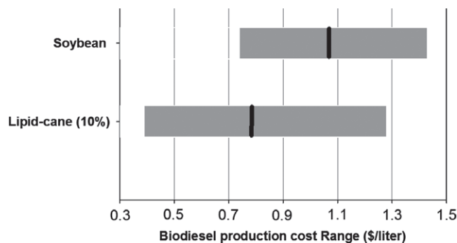
Figure 7. Accumulated uncertainties of the sensitivity parameters on the biodiesel production cost. The base values are included for reference as a vertical bar.
