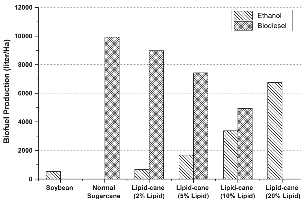
Figure 8. Biofuel production per hectare of land use by soybeans and lipid-cane. The soybean yield was assumed to be 2.8 MT/ha, and the lipid-cane biomass yield was assumed to be 110 MT/ha. The soybean moisture content was 13%, while the cane moisture content was 70%.
