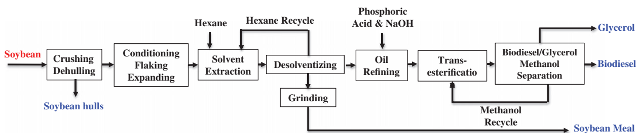
Figure 2. Flow diagram of soybean biodiesel process.
