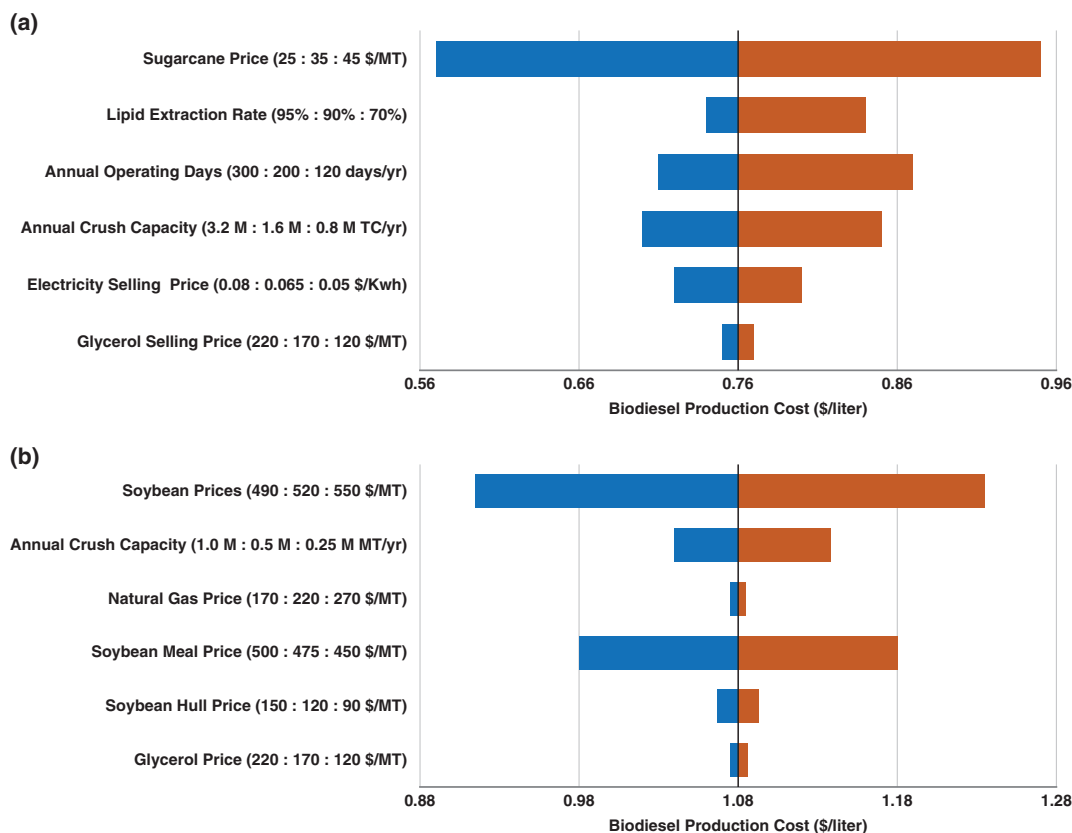
Figure 6. Sensitivity of biodiesel production cost to different parameters. (a) Lipid-cane process; (b) Soybean process. The numbers in brackets in Y-axis are the potential low, base and high values of each parameter.
