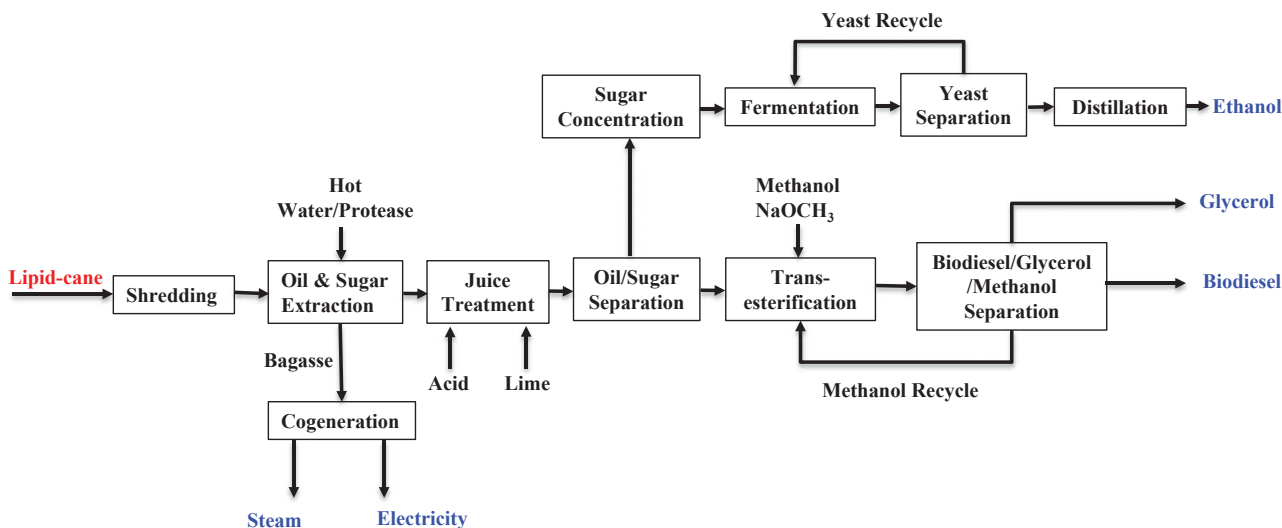
Figure 1. Flow diagram of the lipid-cane process.
