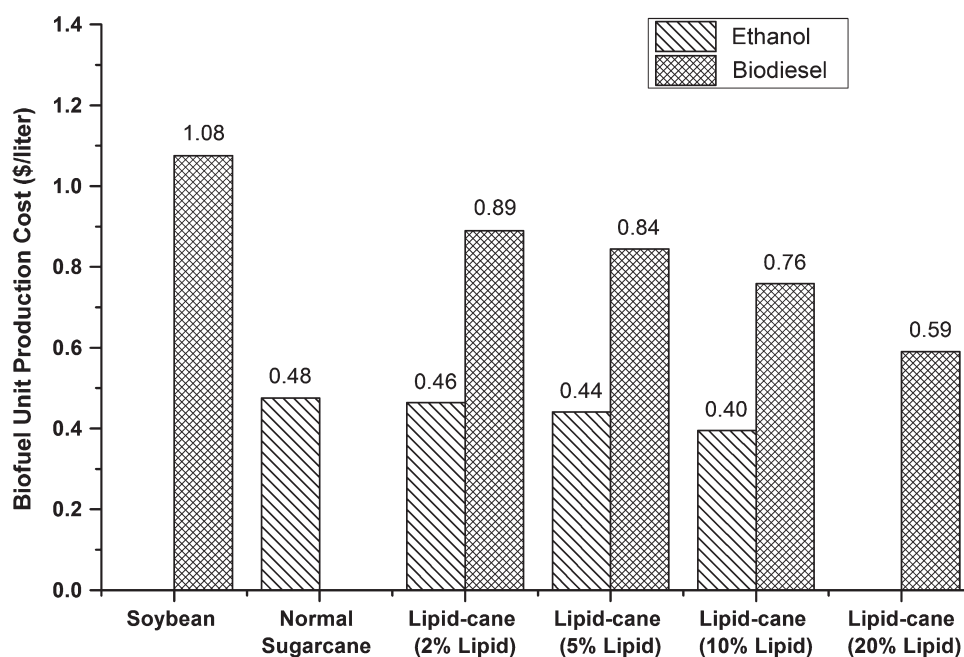
Figure 4. Biofuel unit production costs from soybean, normal sugarcane, and lipid-cane.
