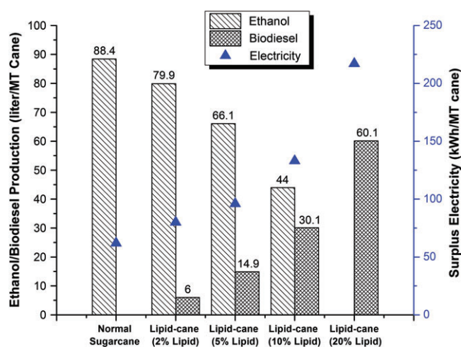
Figure 3. Main product and coproduct (surplus electricity) yields from each MT of normal sugarcane and lipid-cane.
