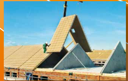
prefab segmenten
