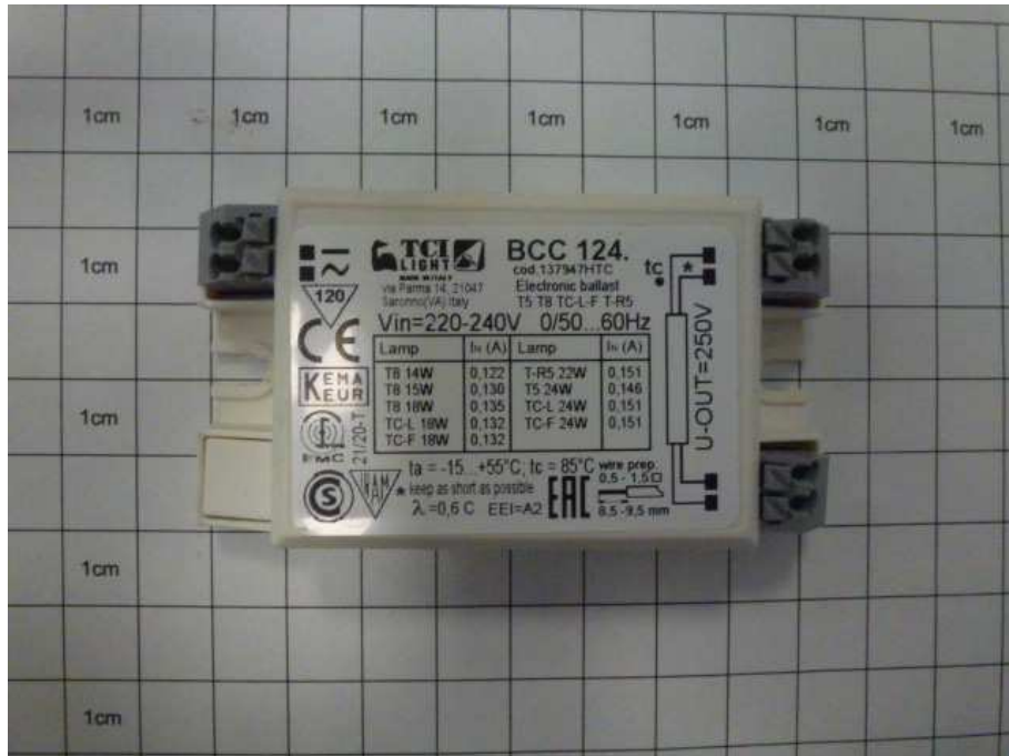
Electronic ballast
