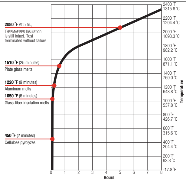
Graph of THERMAFIBER Insulation performance in fire test controlled in accordance with ASTM E119 time-temperature relationship shows superior fire characteristics of THERMAFIBER Insulation products.
