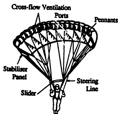
Rear Suspension Lines have not been shown
