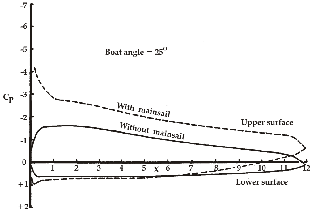
Figure 16. Pressure distribution for jib with and without the main being present.
