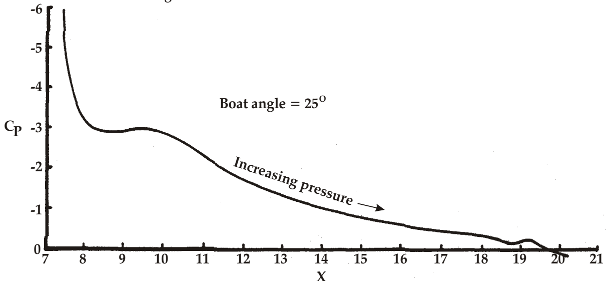
Figure 12. Upper surface pressure distribution about mainsail alone.
