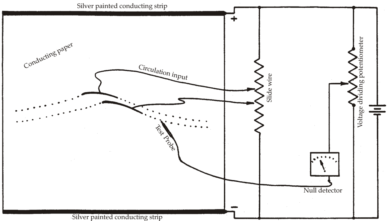
Figure 7. Diagram of analog field plotter.
