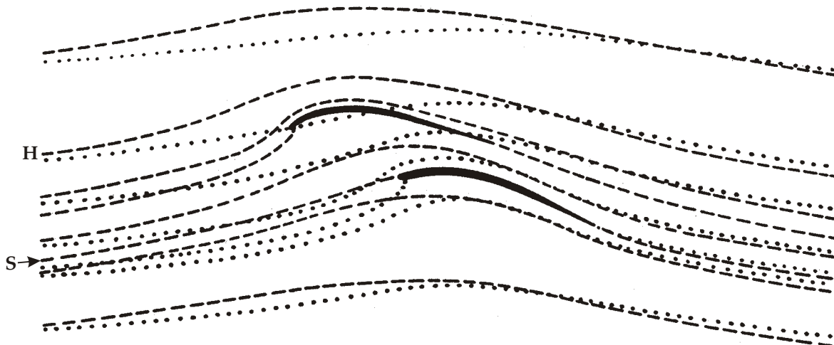
Figure 13. Streamlines about jib and mainsail together. Dashed lines are streamlines with both sails. Dotted lines are when the mainsail was used alone.
