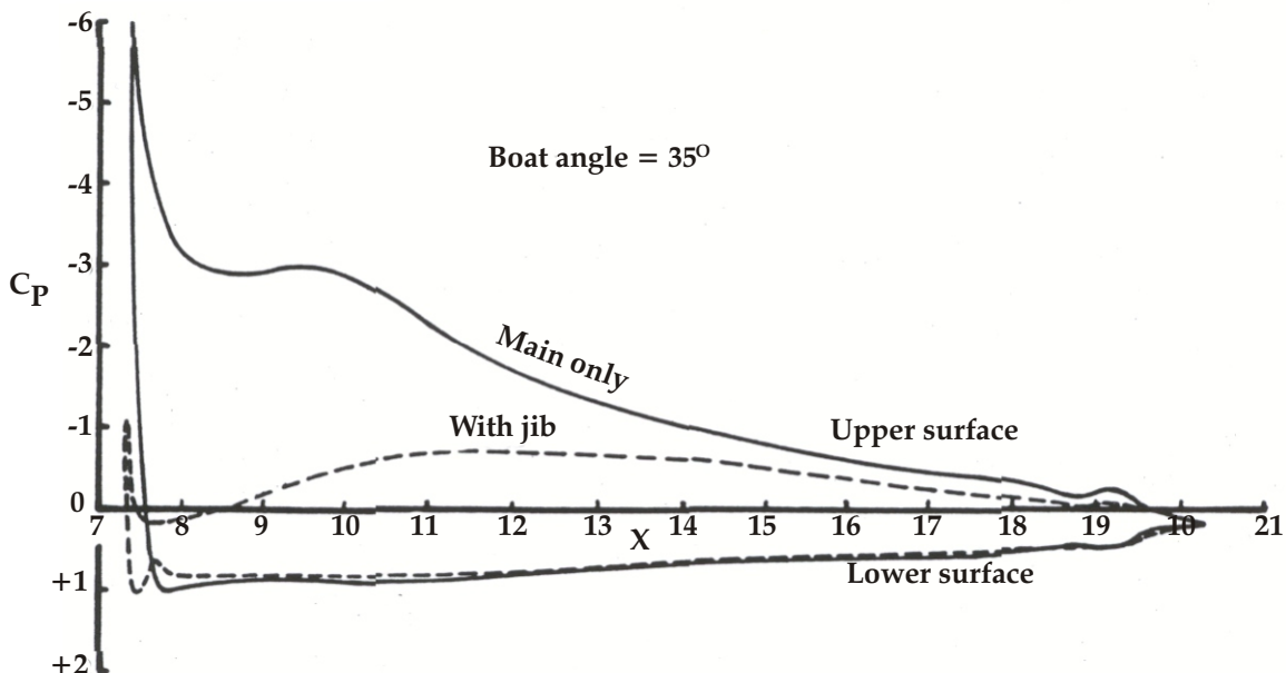
Figure 14. Pressure distribution for mainsail when jib is used. The mainsail in this example could have been trimmed closer to the centerline of the boat to load it up more, but still be able to avoid separation.
