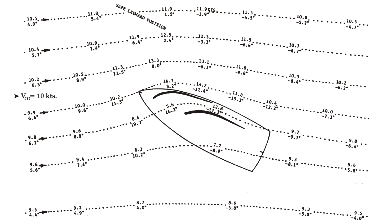
Figure 17. Streamlines about jib and mainsail showing local wind speeds and flow angles.
