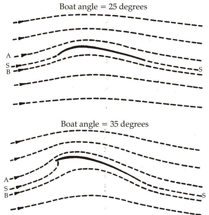
Figure 8. Streamlines about single airfoil.
