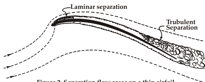
Figure 2. Separation flow areas on a thin airfoil.
