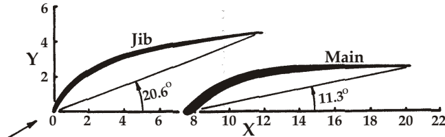
Figure 10. Plot of airfoils used in study.
