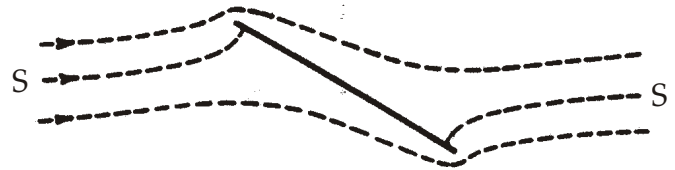
Figure 4. Flow field without circulation (no viscosity).
