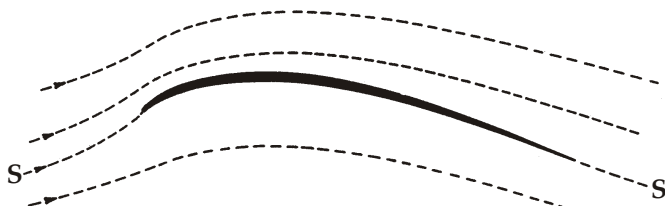
Figure 3. Streamlines about a thin airfoil with boundary layer and separation neglected.
