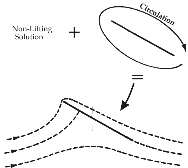
Figure 5. Superposition of circulation and non-circulation solution to give lift.
