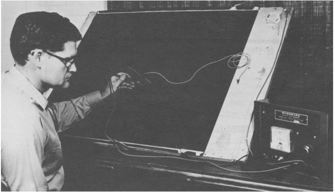
Figure 6. Analog field plotter equipment.
