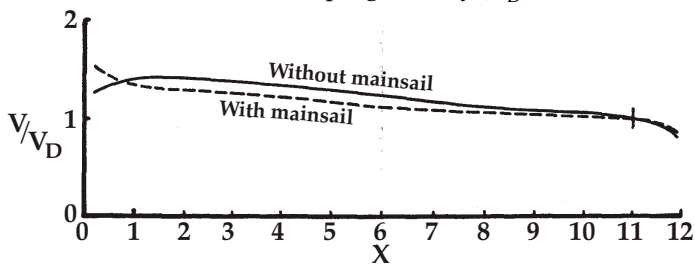
Figure 16. Velocity distribution for jib when normalized by the trailing edge dumping velocity.
