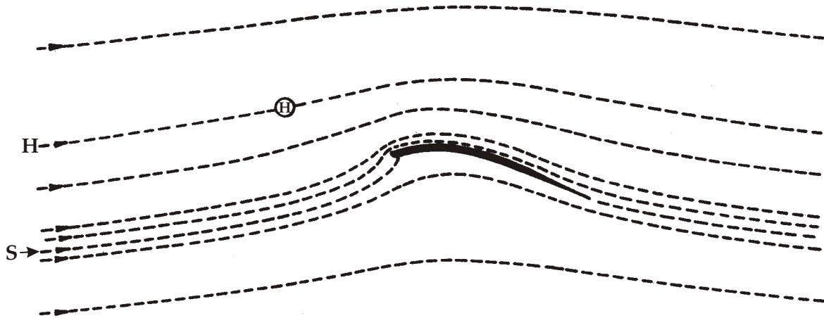
Figure 11. Streamlines about mainsail alone.
