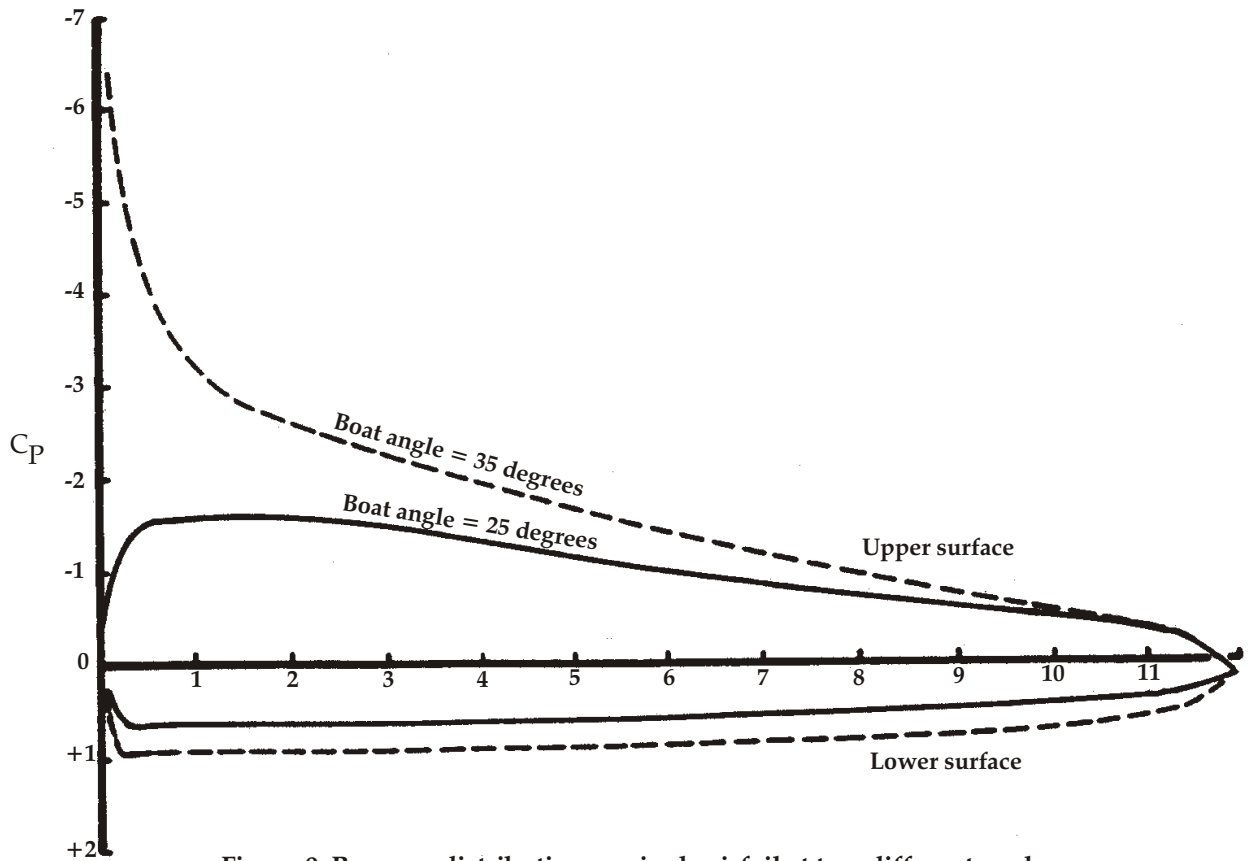
Figure 9. Pressure distribution on single airfoil at two different angles.
