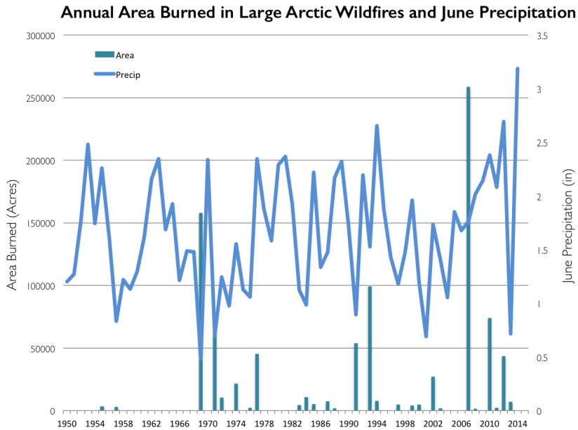
Figure A6. Area burned by large wildfires each year across the Arctic region of Alaska and average June precipitation.
