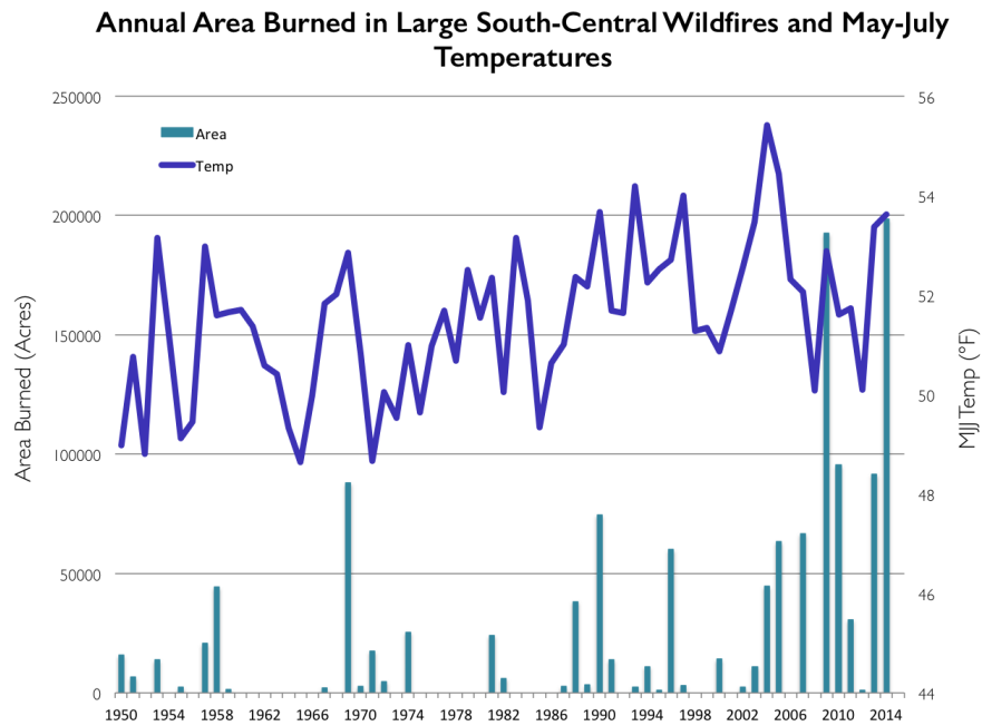
Figure A3. Area burned by large wildfires each year in South-Central region of Alaska and average annual May-June-July (MJJ) temperatures.
