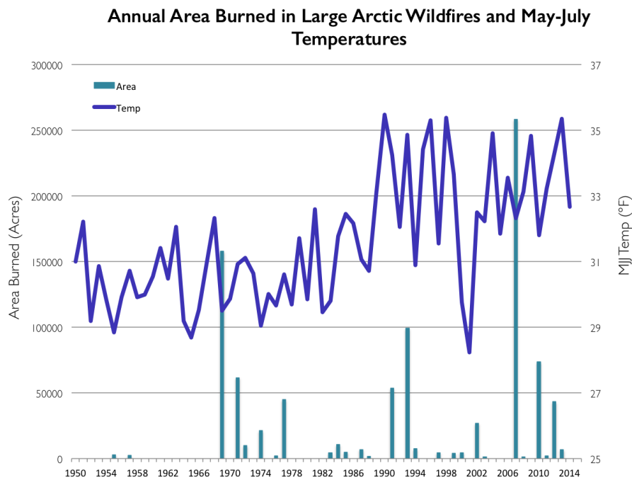
Figure A4. Area burned by large wildfires each year in Arctic region of Alaska and average annual May-June-July (MJJ) temperatures.
