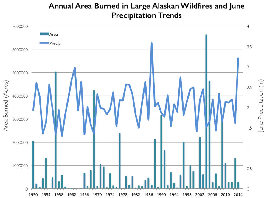
Figure A5. Area burned by large wildfires each year across all regions in Alaska and average June precipitation.
