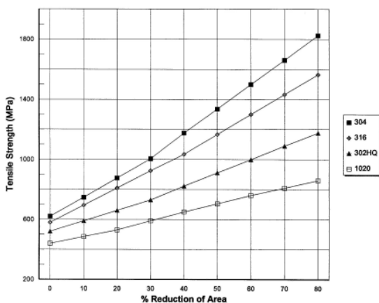
Figure 17 Effect of Cold work on tensile strength of stainless steels. Values are typical for cold drawn wire.
