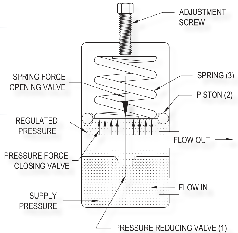
PRESSURE REGULATOR SCHEMATIC SHOWING FORCES ACTING ON THE INDIVIDUAL ELEMENTS
