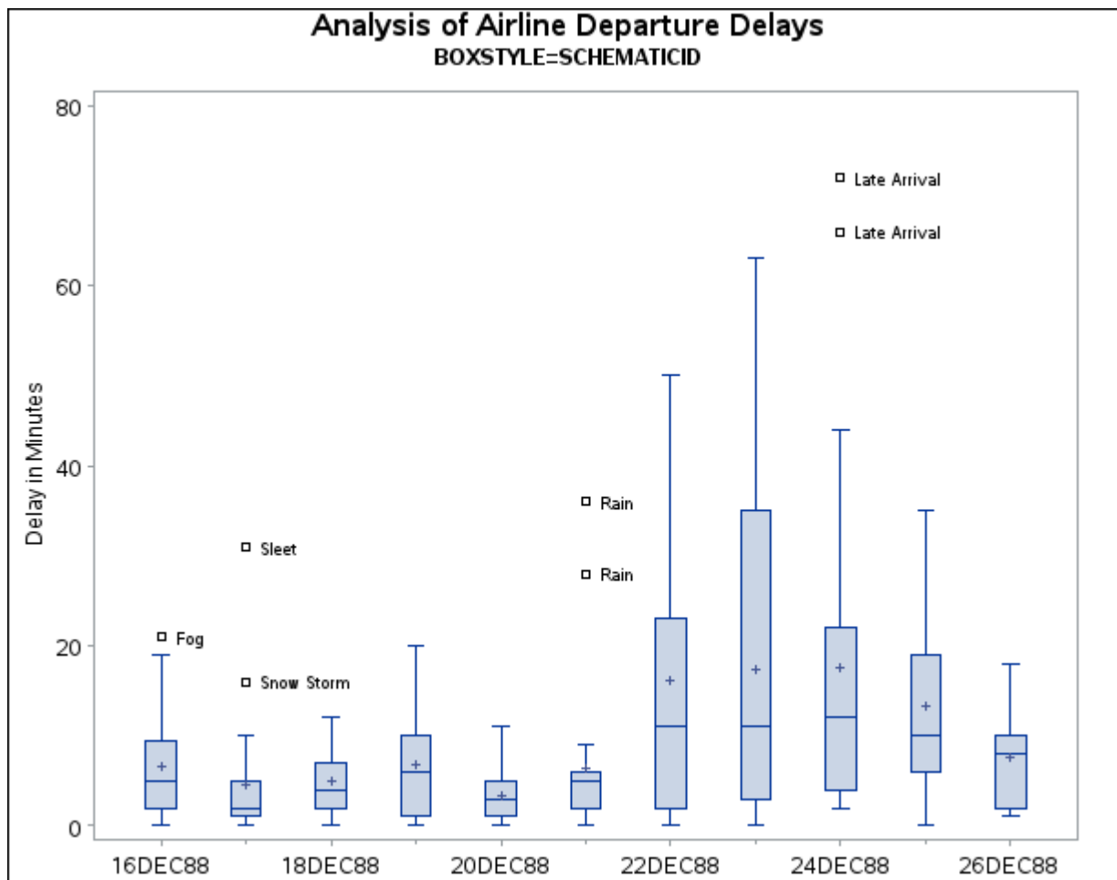
Output 28.3.3 BOXSTYLE=SCHEMATICID
