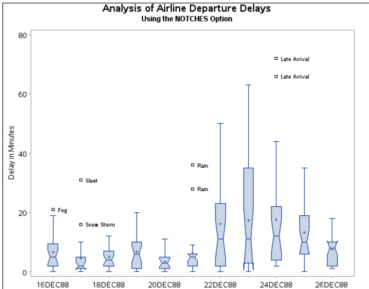
Output 28.4.1 Notched Side-by-Side Box-and-Whiskers Plots
