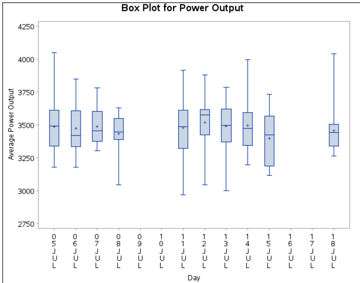
Figure 28.10 Box Plot with Continuous Group Variable
