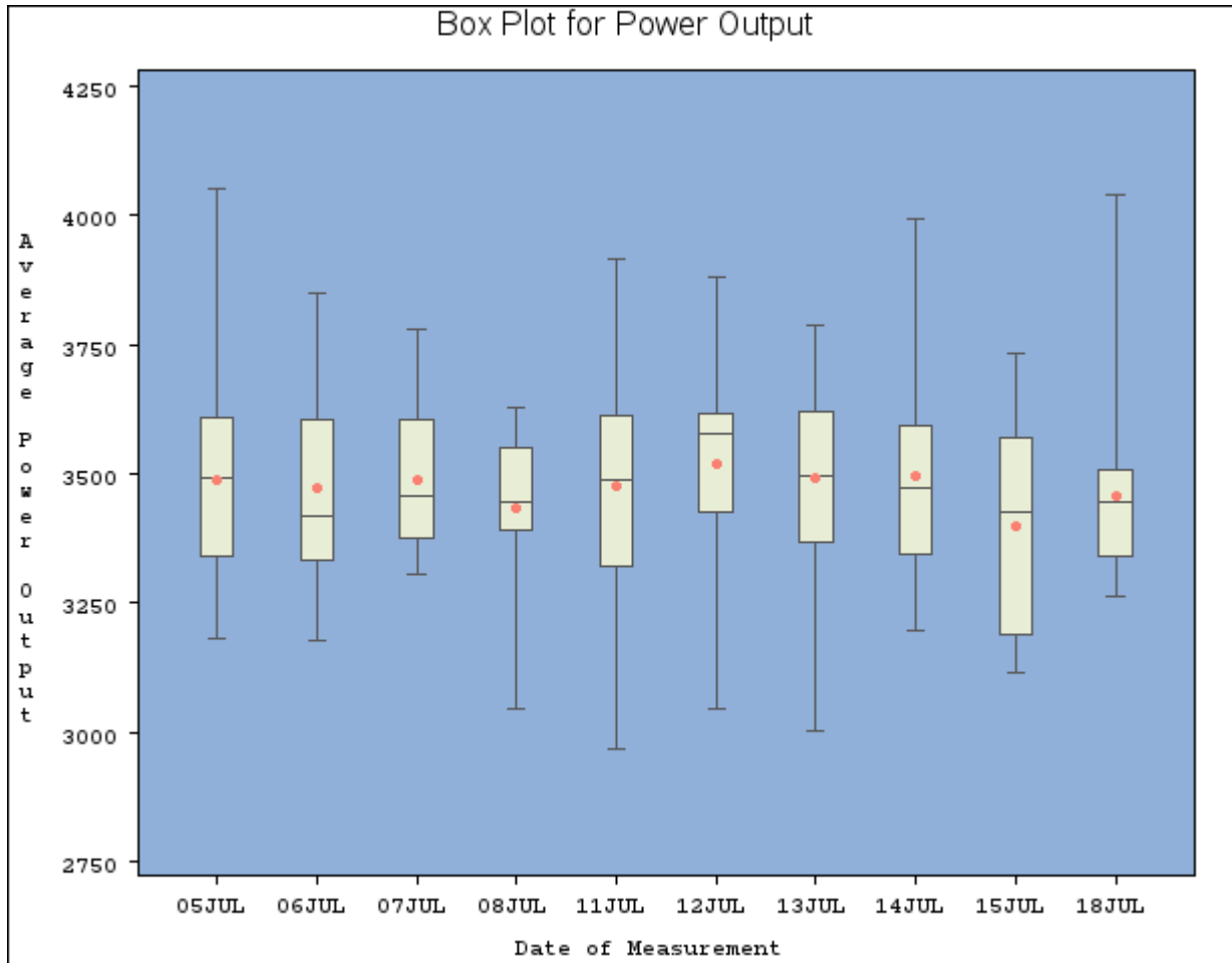
Figure 28.3 High-Resolution Box Plot with NOGSTYLE
