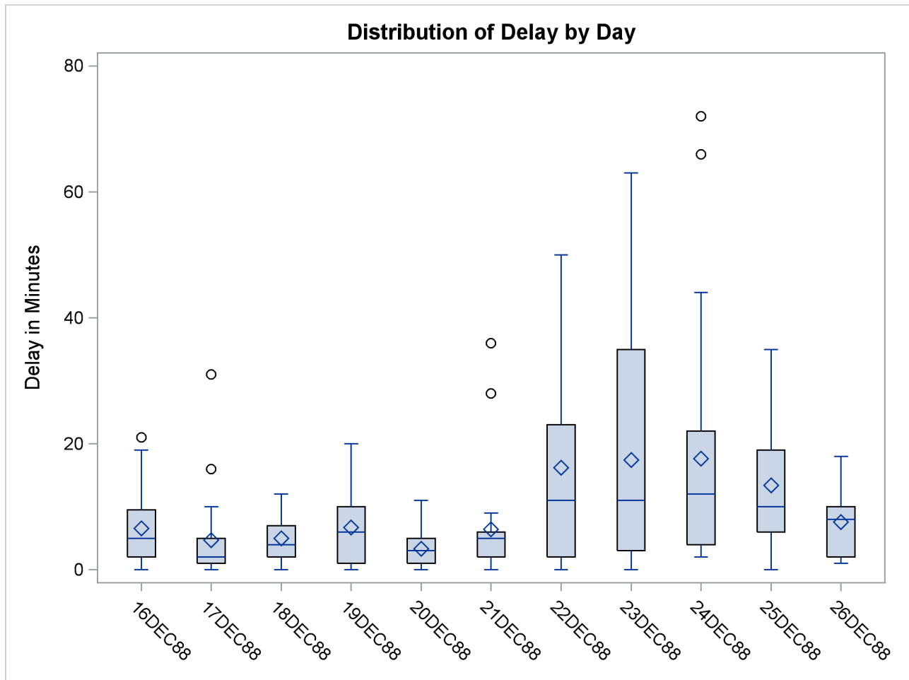
Output 28.6.1 Box Plot Produced Using ODS Graphics
