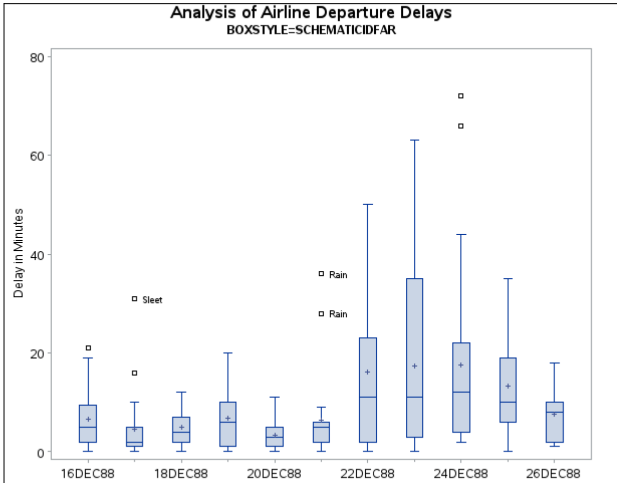
Output 28.3.4 BOXSTYLE=SCHEMATICIDFAR
