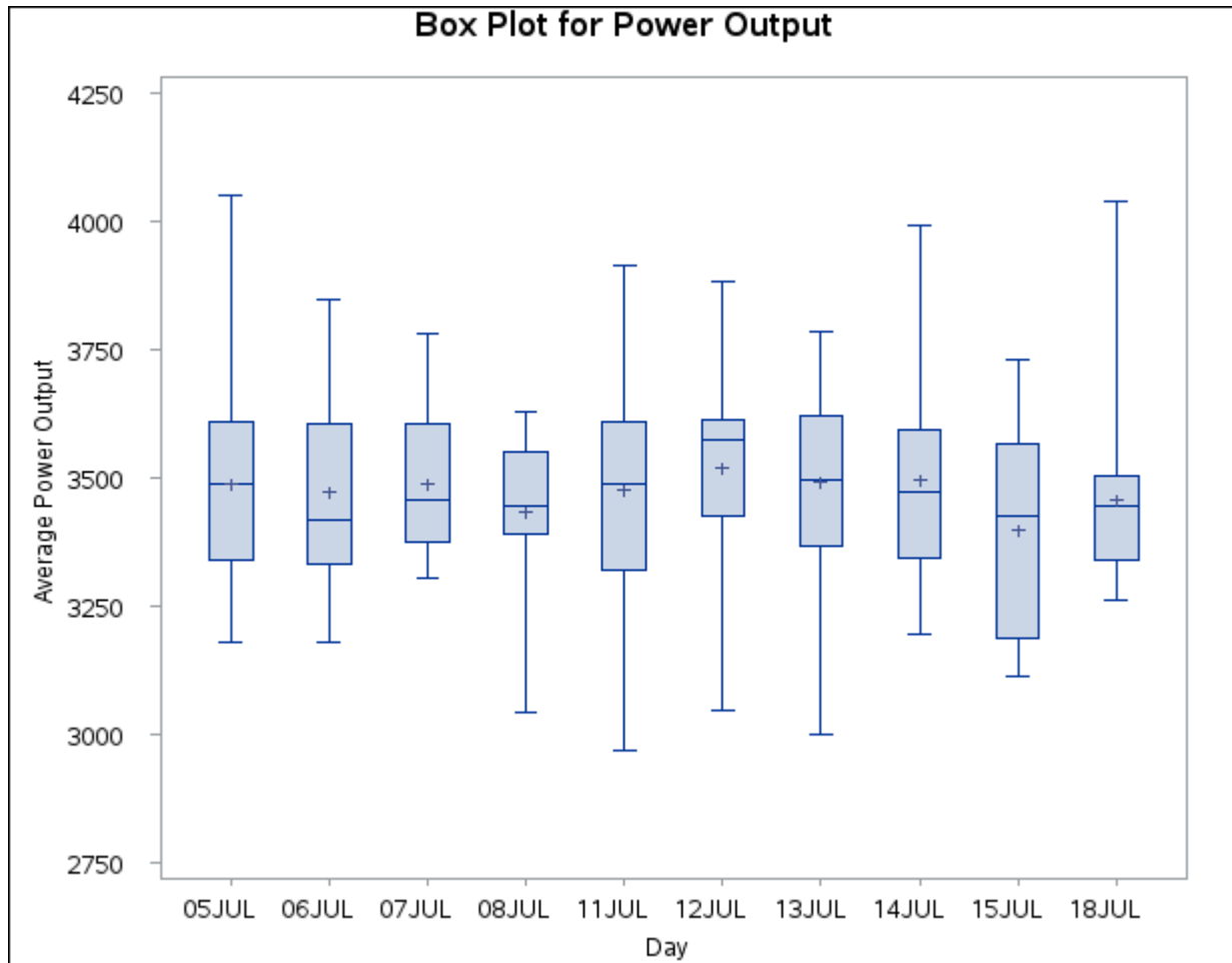
Figure 28.1 Box Plot for Power Output Data
