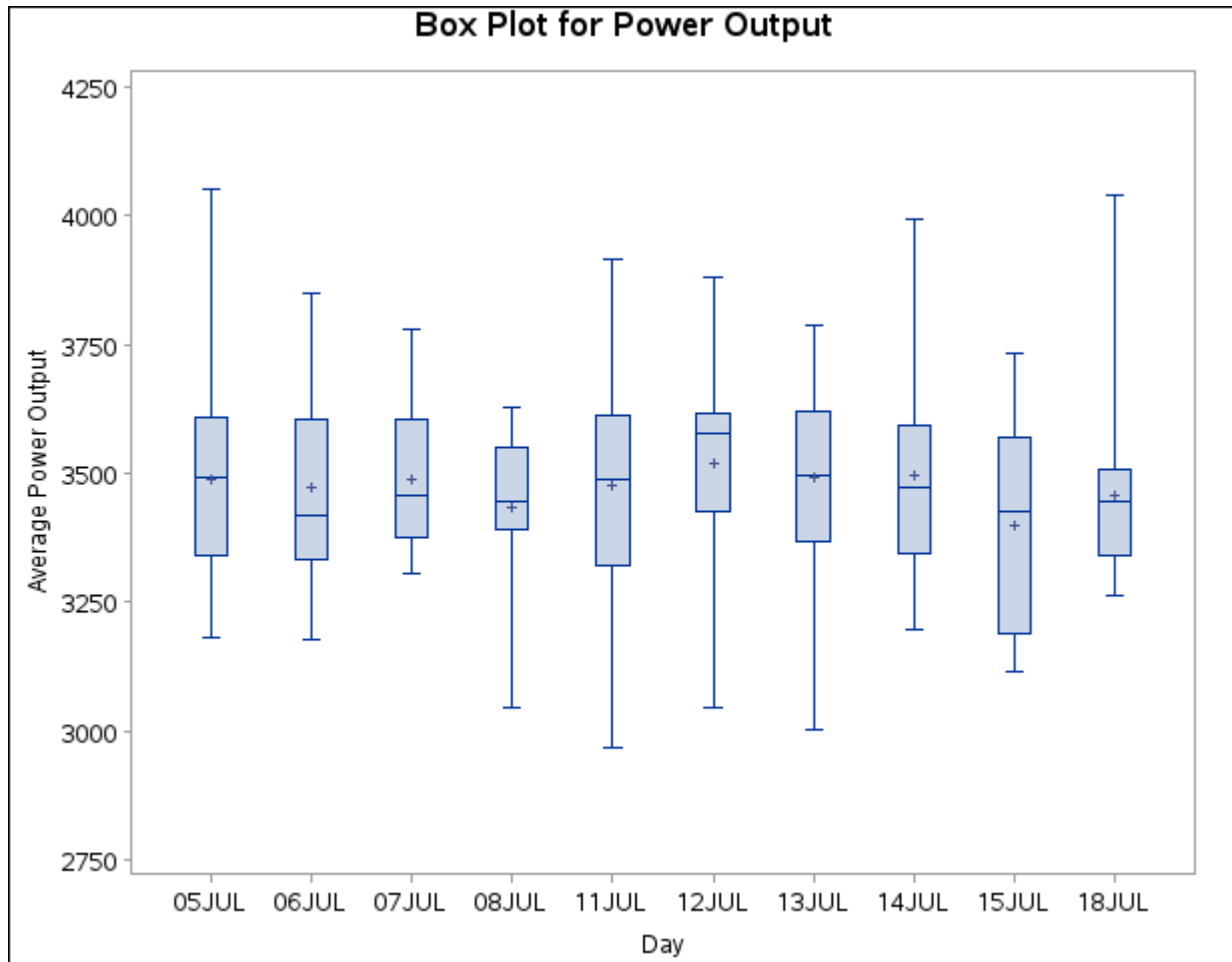
Figure 28.9 Box Plot with Discrete Group Variable
