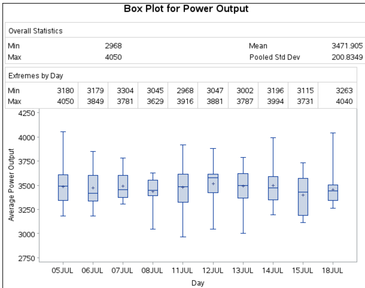
Output 28.1.1 Box Plot with Insets
