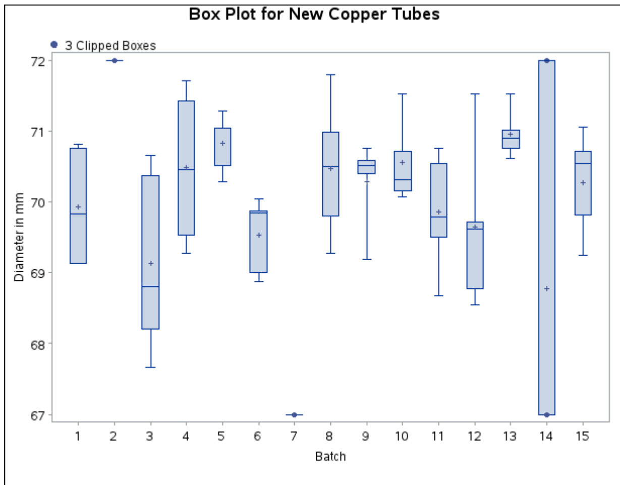
Figure 28.18 Box Plot Using Clipping Options
