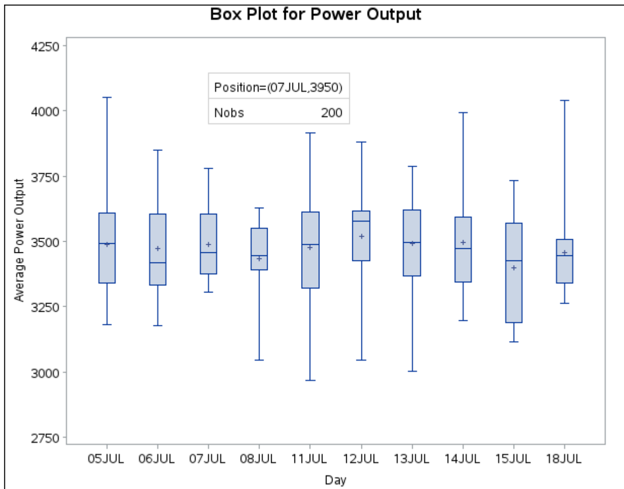
Figure 28.13 Inset Positioned Using Data Unit Coordinates
