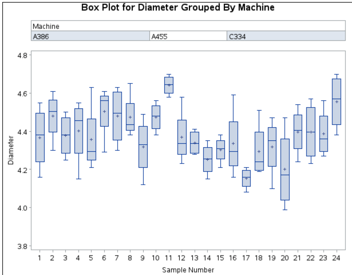
Figure 28.15 Box Plot Using a Block Variable
