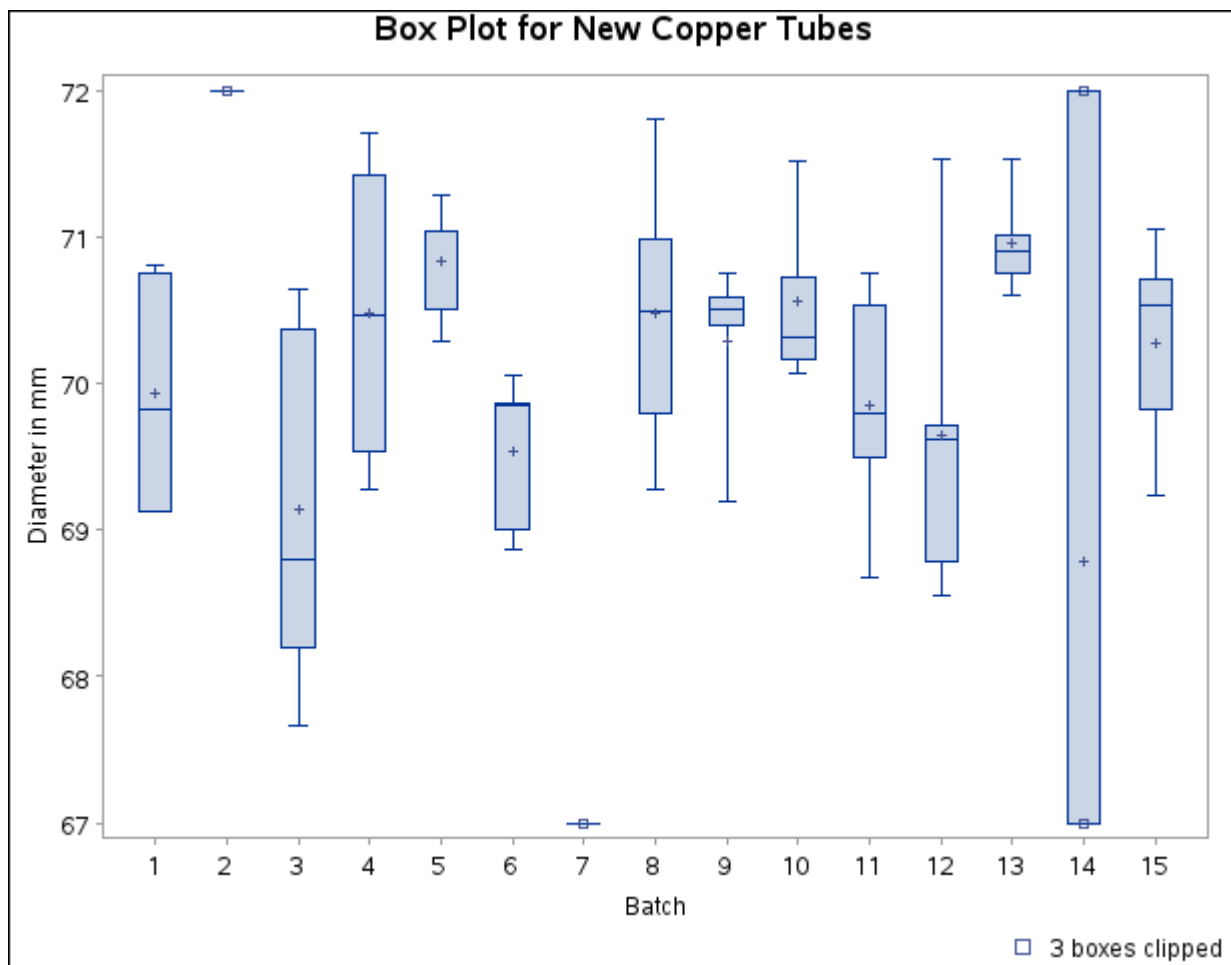
Figure 28.17 Box Plot with Clip Factor of 1.5
