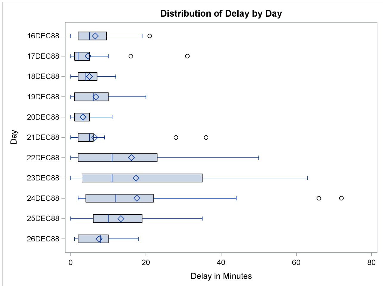
Output 28.6.2 Horizontal Box Plot
