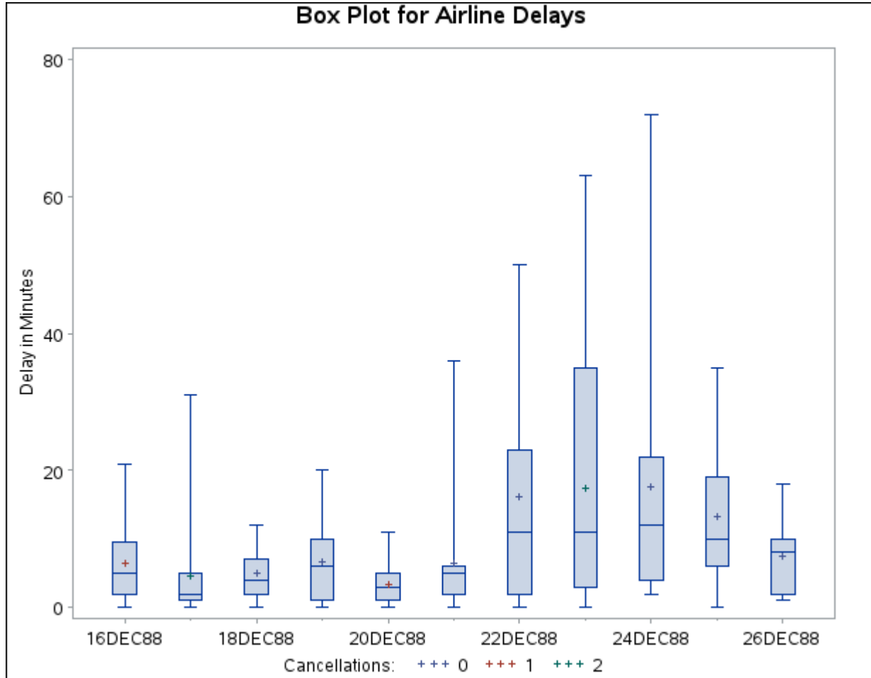
Output 28.2.1 Box Plot for Airline Data
