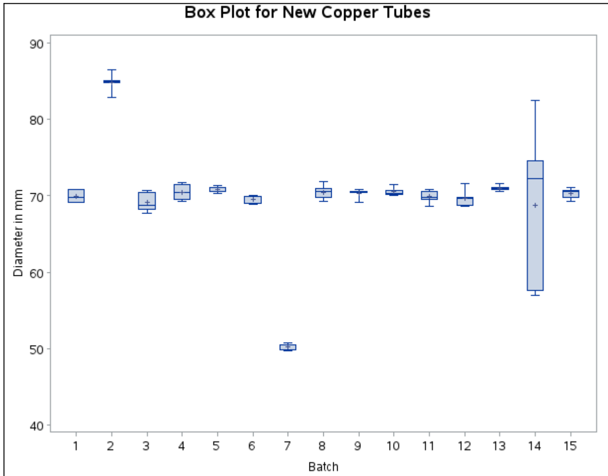
Figure 28.16 Compressed Box Plots
