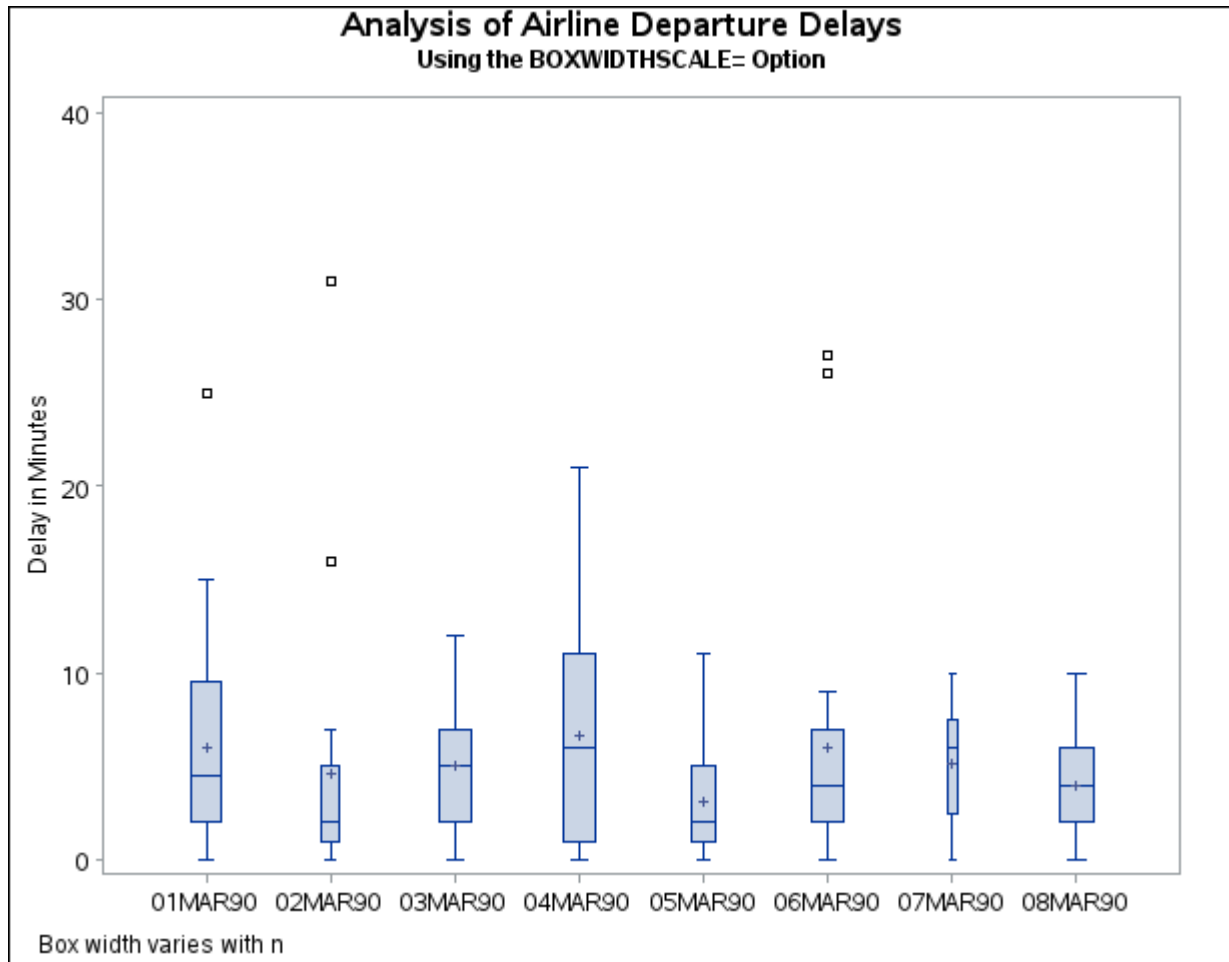
Output 28.5.1 Box Plot with Box-and-Whiskers Plots of Varying Widths
