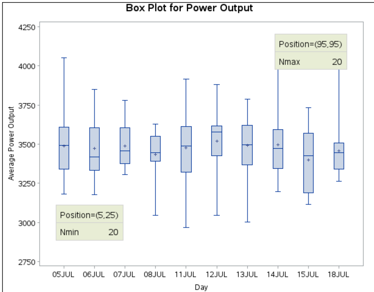
Figure 28.14 Inset Positioned Using Axis Percent Unit Coordinates
