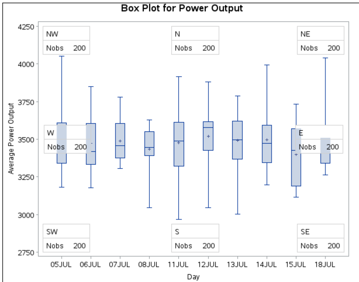
Figure 28.11 Insets Positioned Using Compass Points
