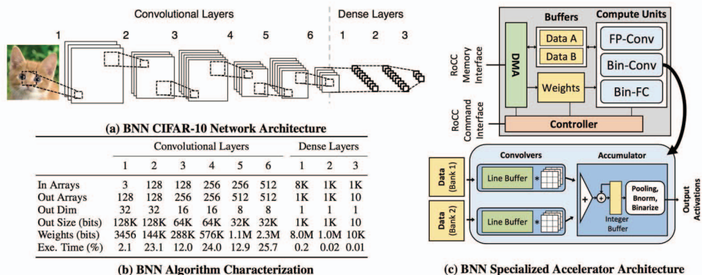
Figure 3. BNN accelerator.
