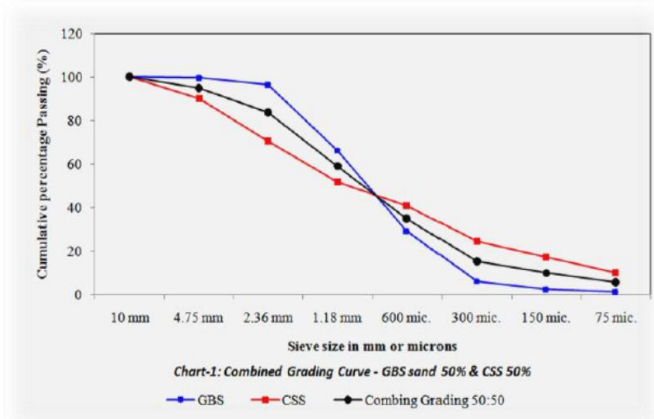
Fig2- Sieve Analysis of Natural Sand and GBS Sand
