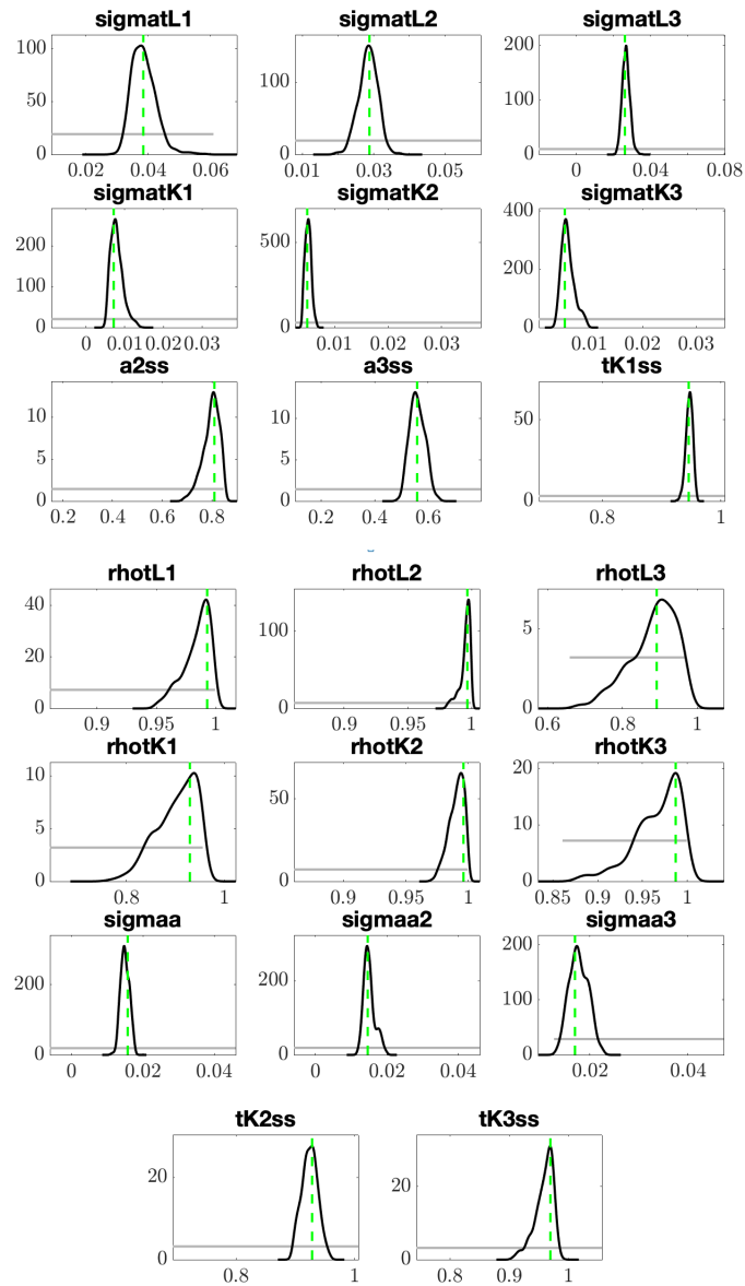
Figure 11: Priors and Posteriors
