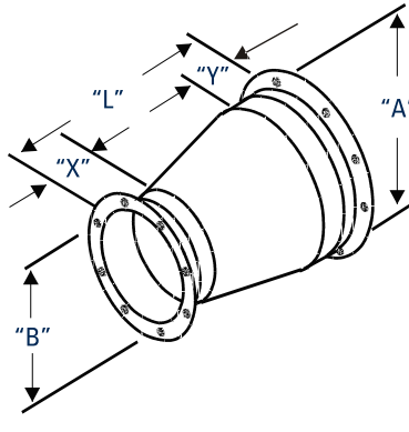
"FLANGED STYLE"
