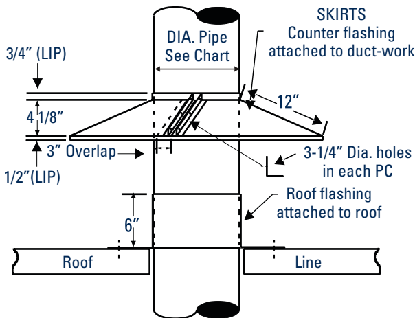
ELEVATION VIEW
