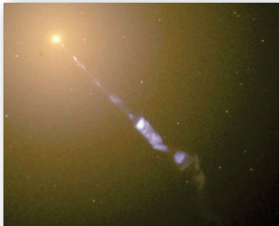
Galaxy M87, exhibiting an energetic jet spanning thousands of light years. The glow is caused by synchrotron radiation, from extremely energetic electrons spiraling along magnetic field lines. The jet was first detected in 1956 by Geoffrey Burbidge, confirming predictions by plasma scientists Hannes Alfvén and Nicolai Herlofson in 1950, and Josif Shklovskii in 1953. Credit: NASA/ESA
