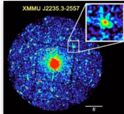
Combining observations by the Very Large Telescope and the XMM-Newton X-ray observatory, astronomers discovered (white inset) a massive cluster of galaxies—“the most distant, very massive structure in the Universe known so far.” According to the announcement by the European Southern Observatory, “The discovery of such a complex and mature structure so early in the history of the Universe is highly surprising.” To state the point more accurately, astronomers had long believed such ‘early’ structure to be impossible. But is this cluster really as distant, massive, and ‘early’ as astronomers’ theoretical assumptions imply? Credit: ESA, XMM-Newton, Mullis et al.
