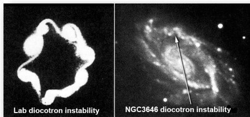
ABOVE LEFT: an image of a ‘diocotron’ instability in a 58-micro-ampere beam of electrons. The enormous scalability of plasma phenomena is evident in the same type of instability in the arms of a galaxy (RIGHT). Credit: LEFT: H. Davis. RIGHT: H. F. Webster.
