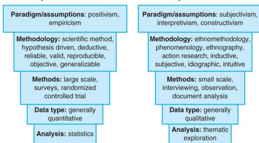
Figure 8.1 Assumptions related to the quantitative and qualitative traditions
