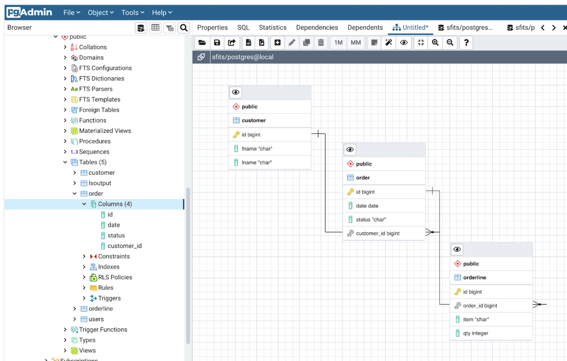
pgAdmin's ERD diagramming Tool
