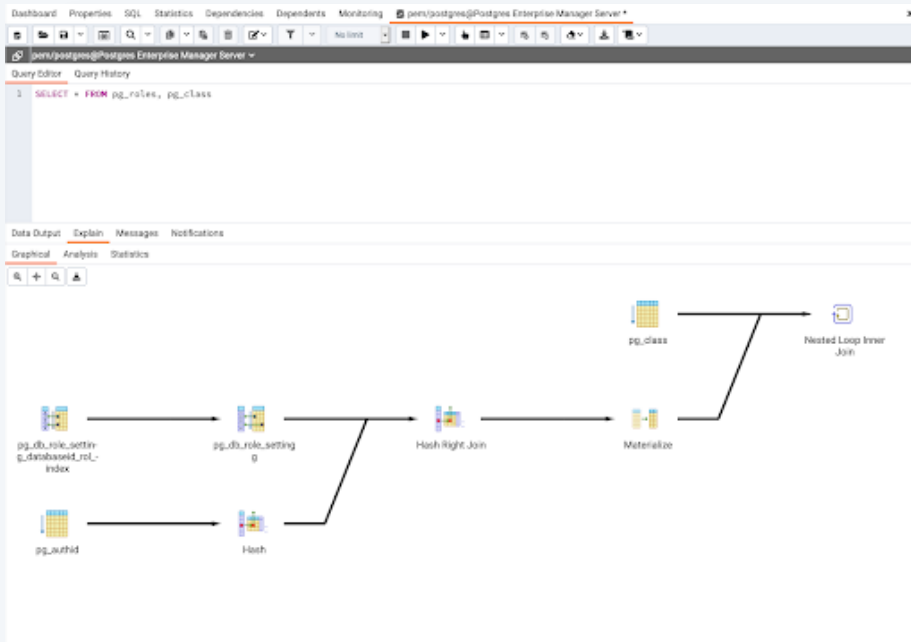
EDB PostgresSQL Enterprise Manager – Query Plan Visualizer
