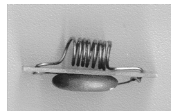
Original trap using receiver components. C = 150pf
