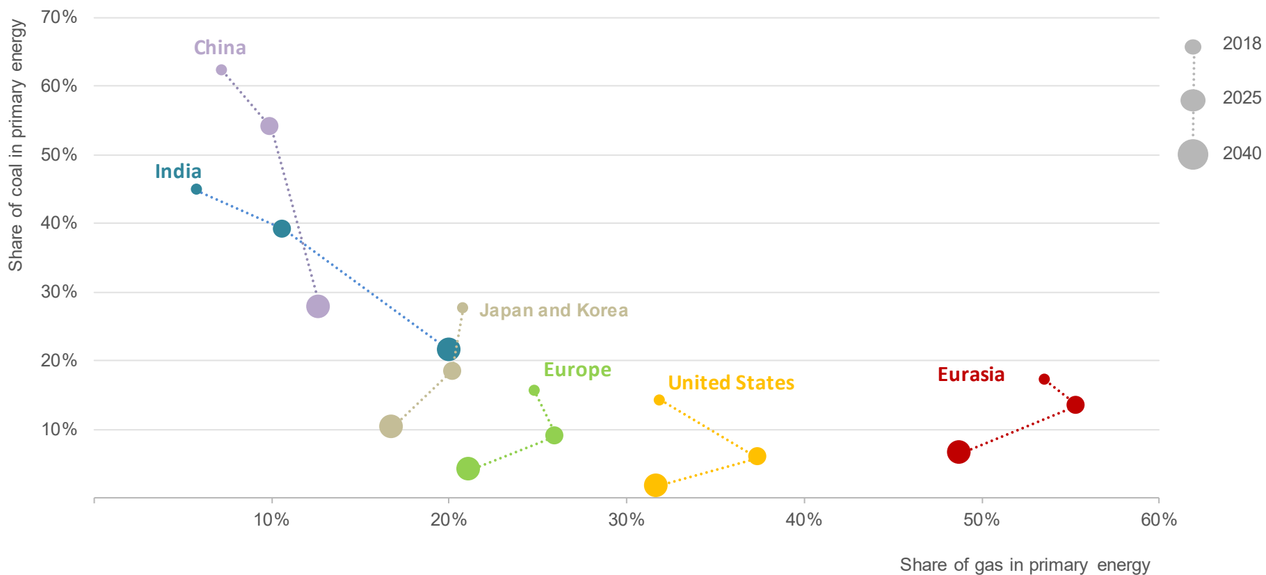
Share of coal and natural gas in primary energy demand in selected regions in the SDS
