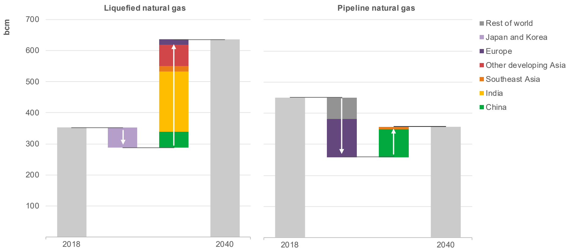
Long-distance natural gas trade by destination in the SDS
