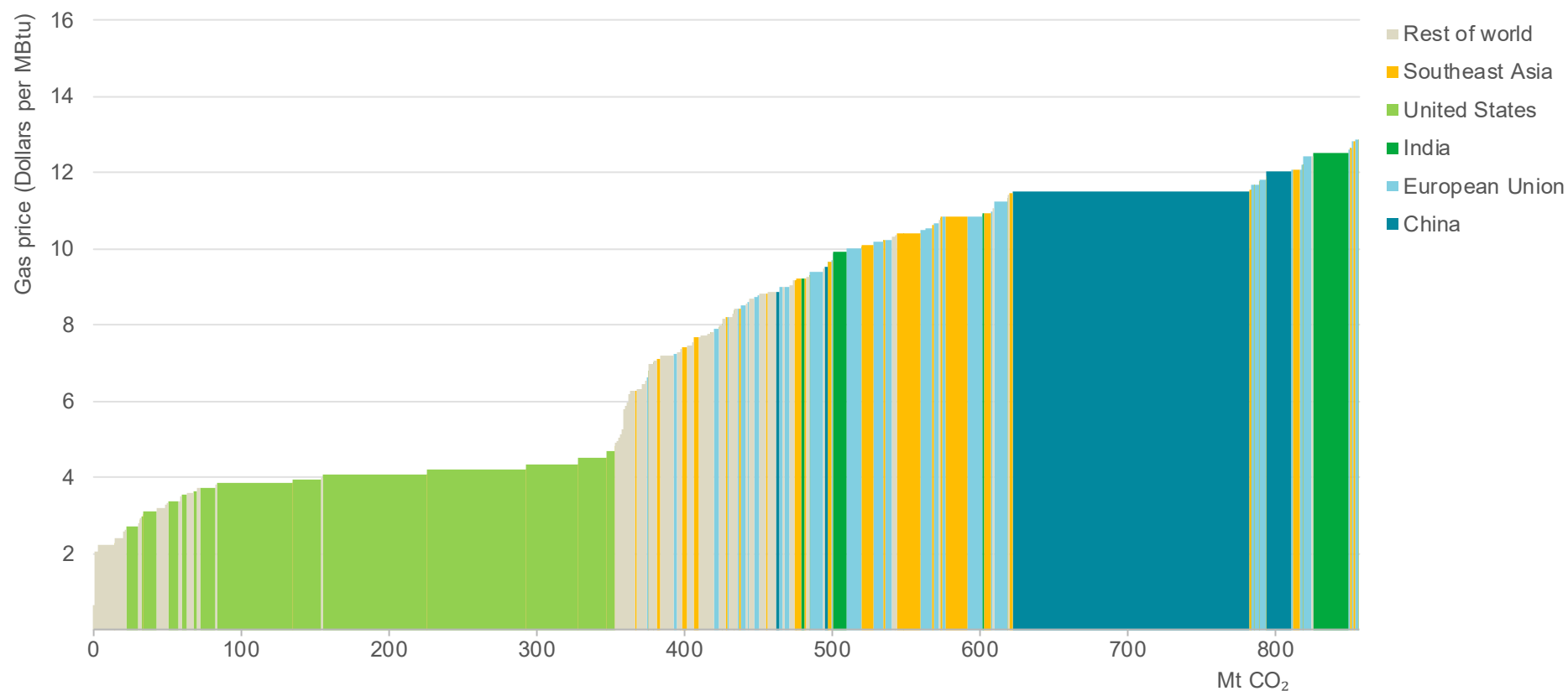
Possible additional CO 2 emissions from gas-to-coal switching in the power sector at higher natural gas prices
