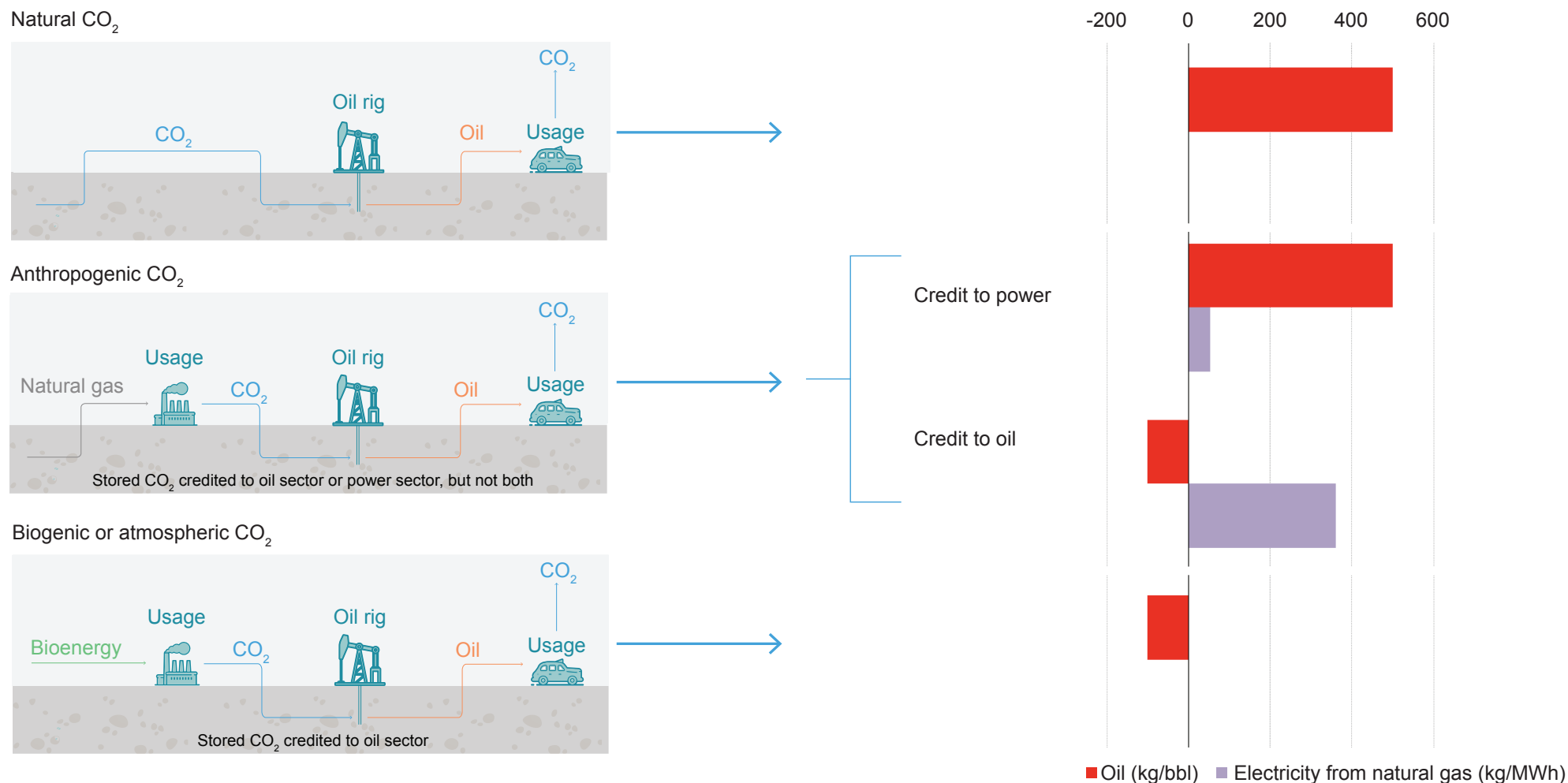
Allocation of CO 2 emissions and credits from CCUS during CO 2 -EOR for different sources of CO 2
