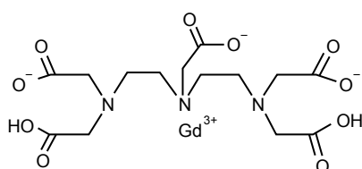
Omniscan (gadodiamide) Linear structure
