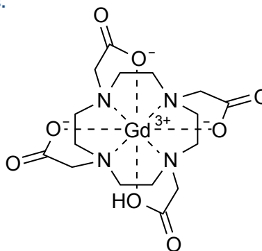
Dotarem (gadoterate meglumine) Macrocyclic structure
