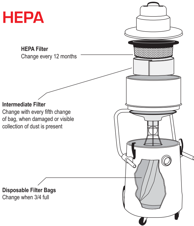
HEPA Filter Wet/Dry Vac Systems - 15 Gal
