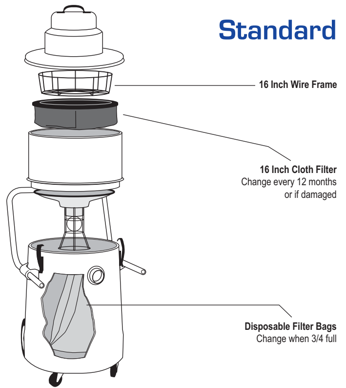
Standard Filter Wet/Dry Vac Systems - 15 Gal
