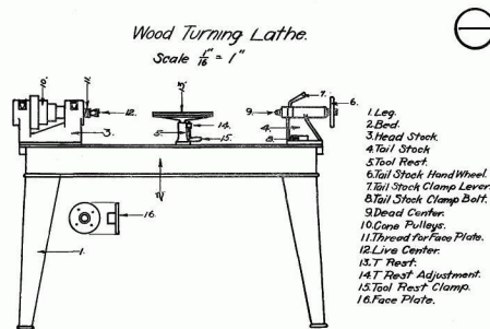
Fig. 1. - Wood Turning Lathe
