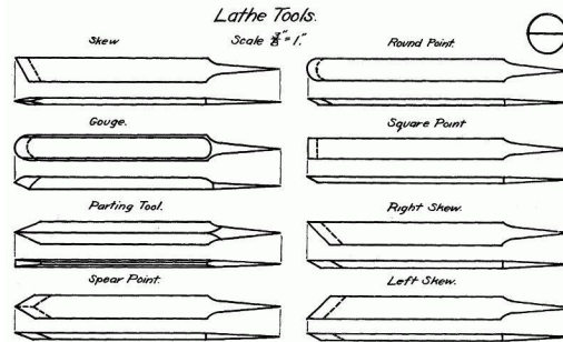
Fig. 2. - Lathe Tools
