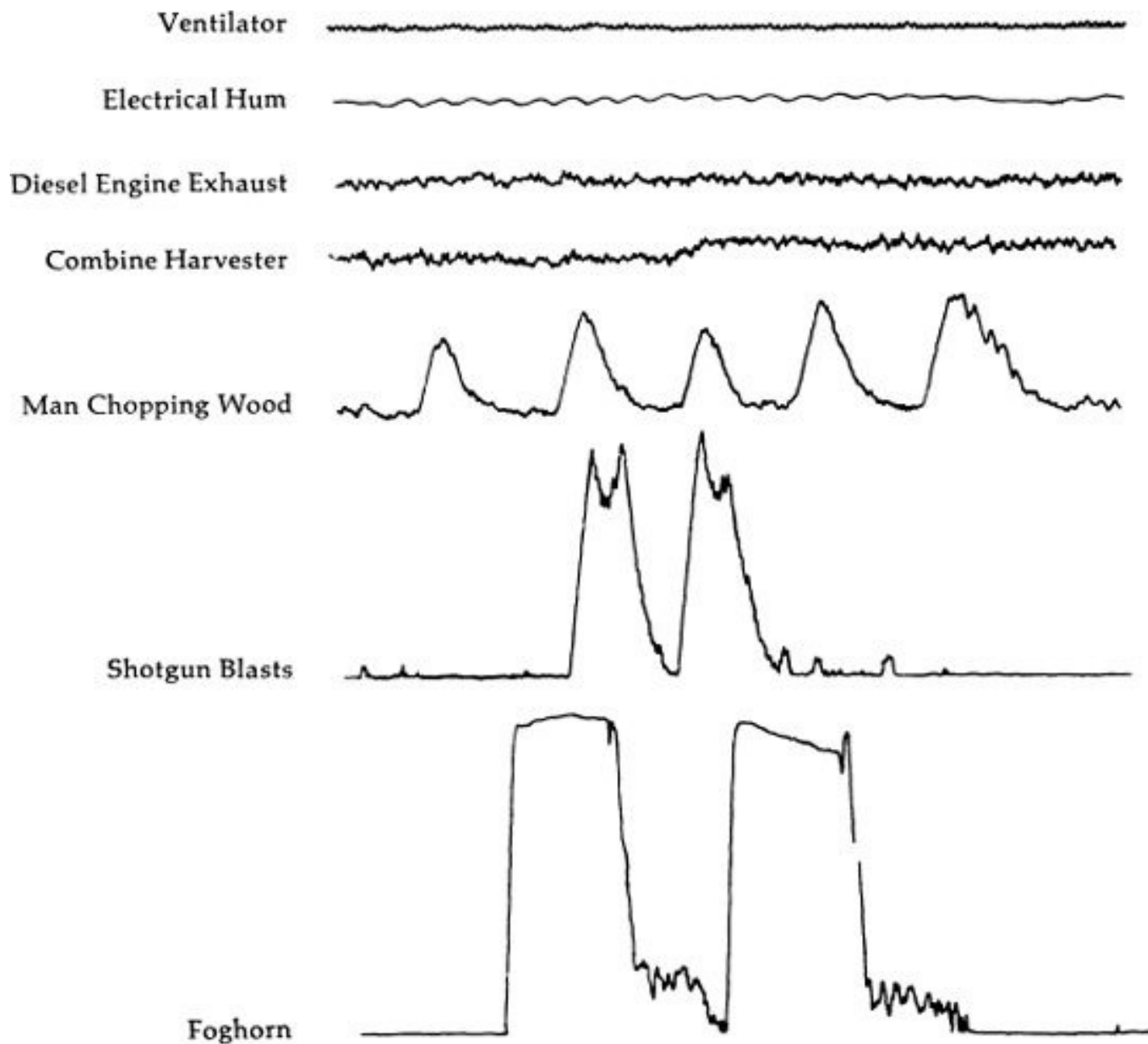
Graphic level recordings of typical flat-line and impact sounds.
