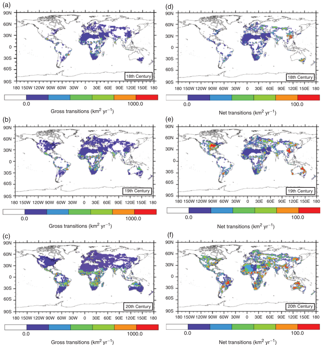
Fig. 7 For simulations with HYDE land-use history, mean annual gross land-use transitions in each 1^{\circ} \times 1^{\circ} grid cell during (a) 18th century, (b) 19th century, and (c) 20th century, and total integrated net land-use transitions in each 1^{\circ} \times 1^{\circ} grid cell during (d) 18th century, (e) 19th century, and (f) 20th century. Note that the scale for gross transitions is 10 times the scale for net transitions.
