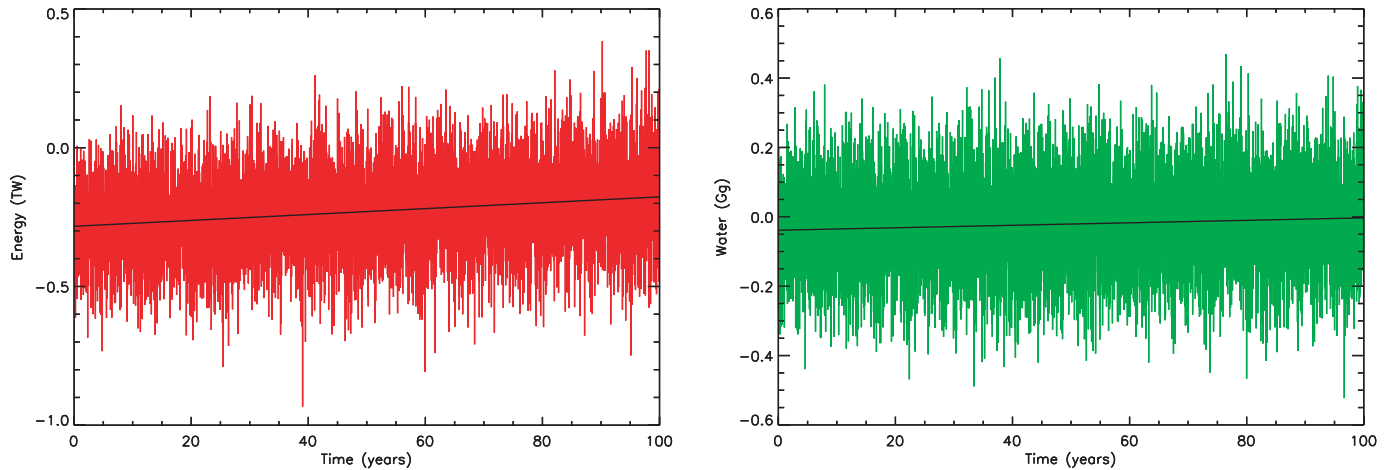
Fig. 9 Model drift relative to the total energy (left) and fresh water (right) at the start of a 100-year run. Black lines indicate a linear least squares fit to the totals.
