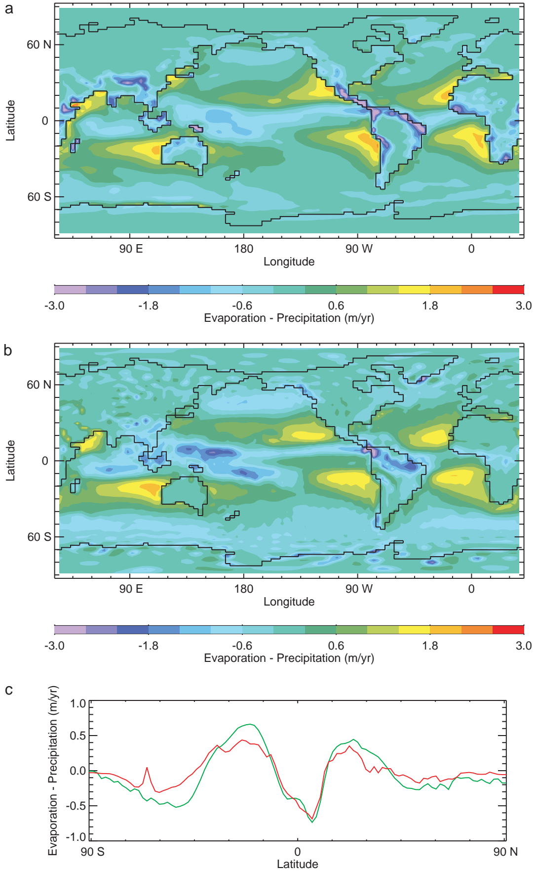
Fig. 25 Annual mean evaporation minus precipitation ( \text{m yr}^{-1} ) for a) model, b) NCEP, c) the zonally-averaged model (red) and NCEP (green) climatologies.
