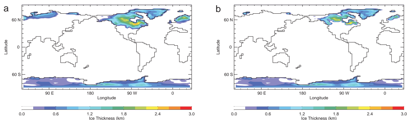
Fig. 43 LGM annually-averaged land ice thickness greater than the present-day bed topography: a) initial condition (reconstruction); and b) at equilibrium after release from the initial condition.
