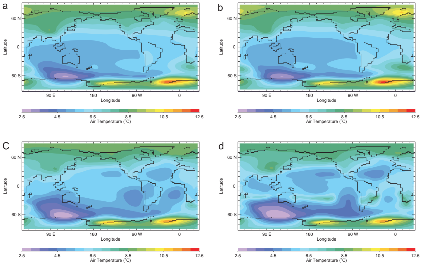
Fig. 32 Surface air temperature change at year 500 (relative to 1998) for the 4 \times \text{CO}_2 equilibrium integrations: a) diffusive moisture transport; b) diffusive moisture transport with wind feedback; c) advective moisture transport; d) advective moisture transport with wind feedback.
