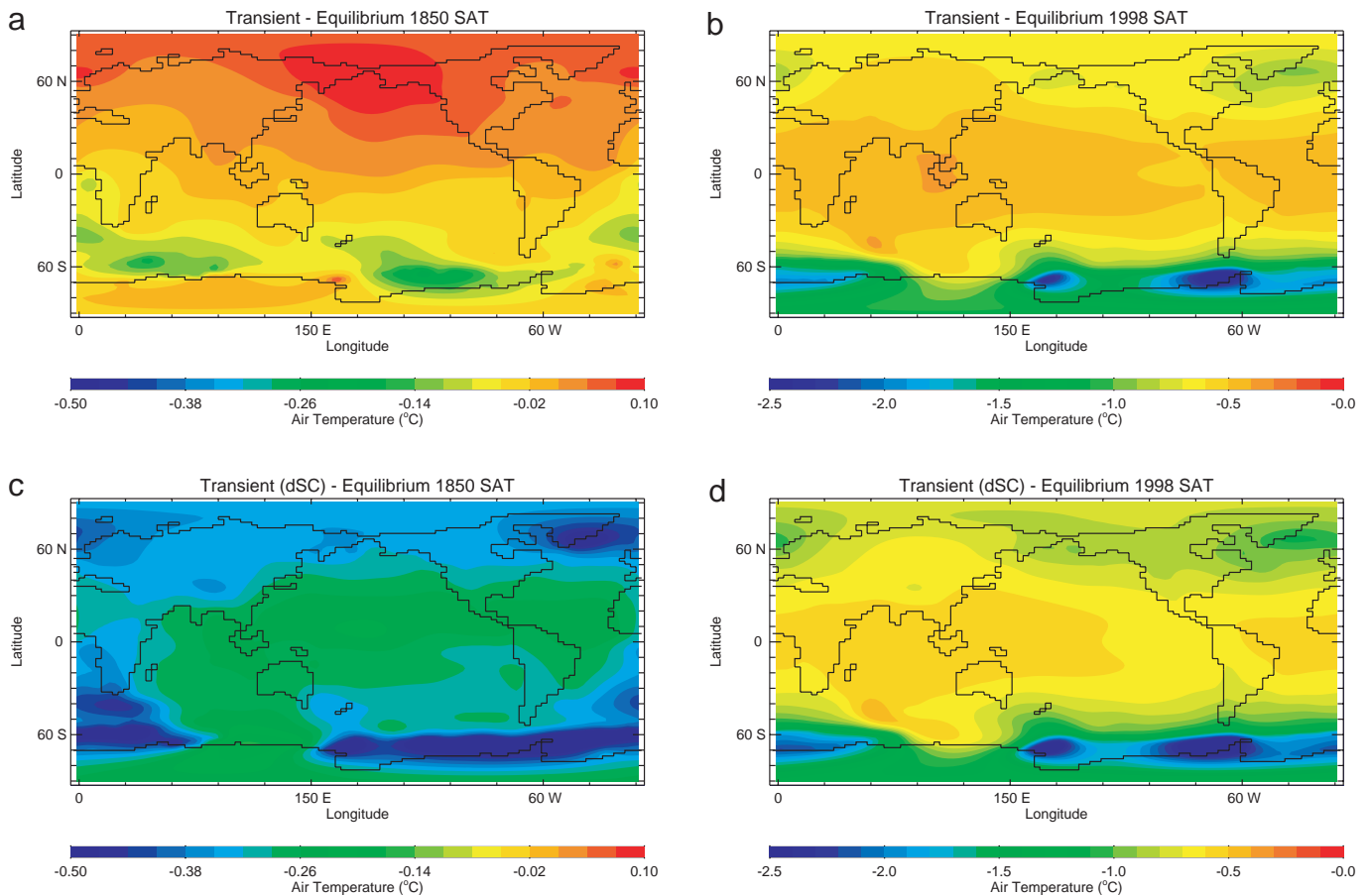
Fig. 47 Surface air temperature (°C) difference between the transient (without varying solar forcing) and equilibrium model simulations at 1850; b) as in a) but at 1998; c), d) as in a), b), respectively, but including varying solar forcing.
