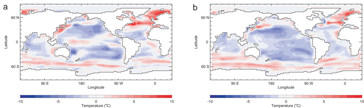
Fig. 42 Anomaly maps showing the difference between the model and CLIMAP Project Members (1976, 1981) sea surface temperature changes between the LGM and the present: a) summer; b) winter.
