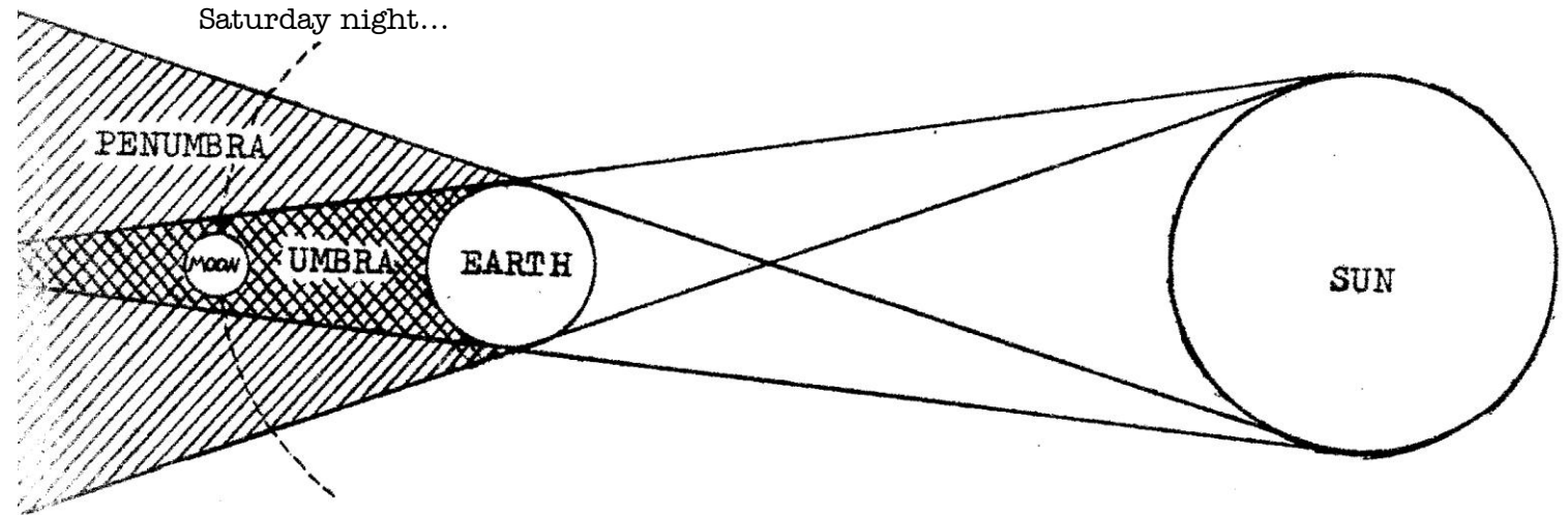
The configuration of a total lunar eclipse (Nothing drawn to scale).
