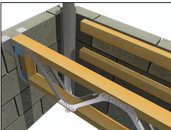
Figure 5: Fixing Around Soil Vent Pipe Using Bearers 38x38 bearers fixed directly to the wall to pick up both floor and ceiling.
