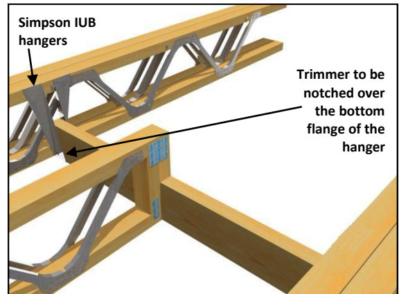
Figure 27: Narrow Opening Detail
