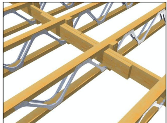
Figure 22: Strongback Splice
