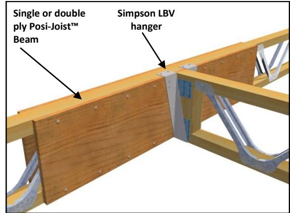
Figure 25: Posi-Joist™ to Posi-Joist™ Connection Plywood nailed to both faces of trimmer beam. Ply/nauling as specified by design
