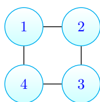
(a) Graph C_4
