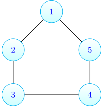
(b) C_5 after applying s .
