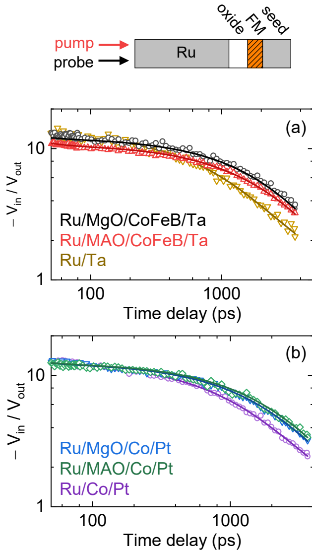
Figure 2. Time-domain thermoreflectance (TDTR) measurement with the pump and probe incident on the Ru surface of the half-MTJ samples with (a) MgO and (b) MgAl 2 O 4 (MAO) tunnel barriers, and of control samples without tunnel barriers. Open symbols are measured TDTR data and solid lines are best-fit.
