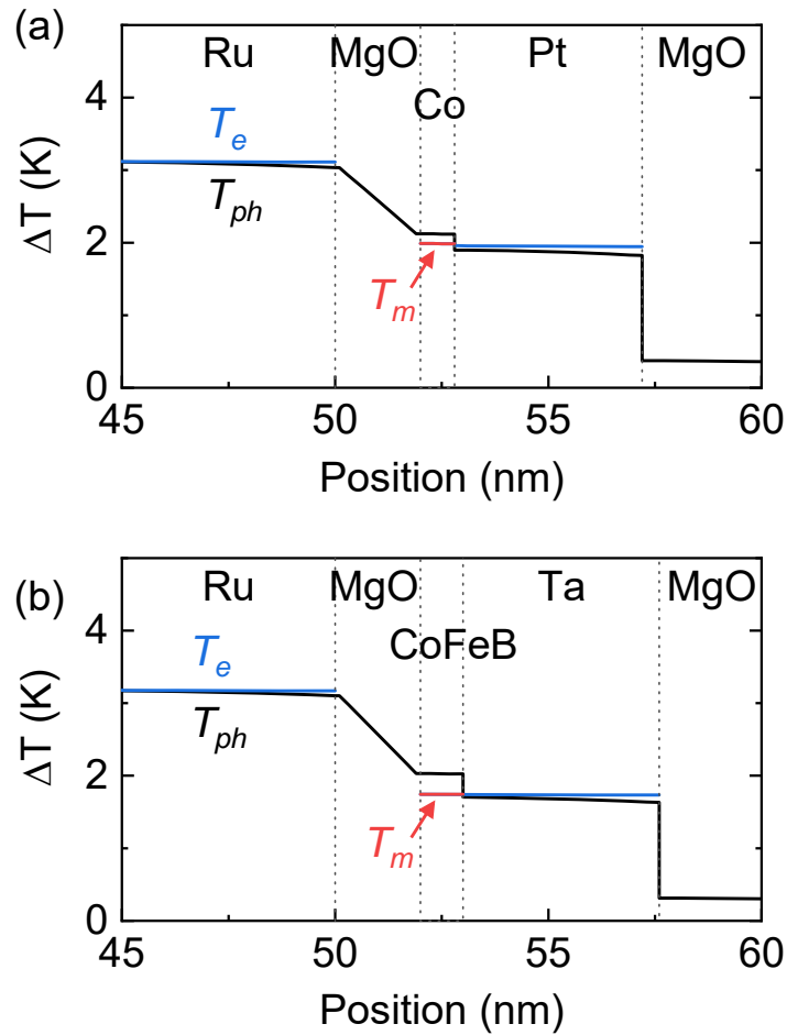
Figure 5. Temperature profiles at delay time of 300 ps in (a) Ru(50)/MgO(2)/Co(0.7)/Pt(4.4)/MgO and (b) Ru(50)/MgO(2)/CoFeB(1)/Ta(4.6)/MgO with the pump beam incident on the Ru surface. The x -axis is the position with respect to the top surface of Ru. Solid lines are the temperatures of electrons (blue), magnons (red), and phonons (black) calculated by the three-temperature model. The temperatures of electrons and magnons appear overlapped (a) in Co and (b) in CoFeB as the differences are < 0.1\% .
