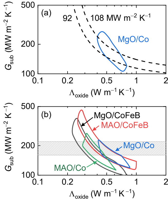
Figure 4. Best-fit of the effective thermal conductivity of oxide tunnel barriers ( \Lambda_{\text{oxide}} ) and the thermal conductance ( G_{\text{sub}} ) of the interface between the seed layer (Pt or Ta) and MgO substrate. (a) Contour (blue solid line) represents the range of \Lambda_{\text{oxide}} and G_{\text{sub}} determined from TR-MOKE on Ru/MgO/Co/Pt sample. Two curves (black dotted line) represents the range of G_{\text{int}} determined from TDTR on the same sample. (b) Ranges of \Lambda_{\text{oxide}} and G_{\text{sub}} for all the samples derived from both TDTR and TR-MOKE. The shaded area represents the range of G_{\text{sub}} determined by TDTR on the control samples without tunnel barriers.
