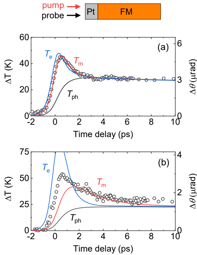
Figure 1. Magnetization dynamics of (a) Co and (b) CoFeB measured by time-resolved quadratic magneto-optic Kerr effect (TR-QMOKE). Sample structures are (a) Pt(2)/Co(10)/sapphire and (b) Pt(2)/CoFeB(6.5)/sapphire. Black symbol is the data obtained by taking a difference of two TR-QMOKE measurements with probe polarizations at +45^\circ and -45^\circ relative to the external in-plane magnetic field, \approx 0.3 T. Solid lines are the best fit of the temperatures of electrons (blue), magnons (red), and phonons (black) at the midpoint of the Co or CoFeB layer calculated by the three-temperature model. The absorbed fluences are (a) 1.2 \text{ J m}^{-2} and (b) 0.8 \text{ J m}^{-2} .
