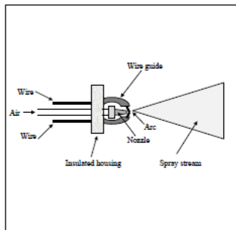
Figure 2-7. Typical two-wire arc spray gun
