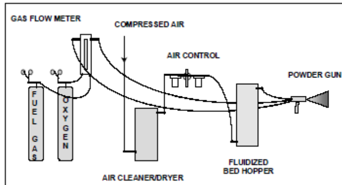
Figure 2-4. Typical combustion powder gun installation
