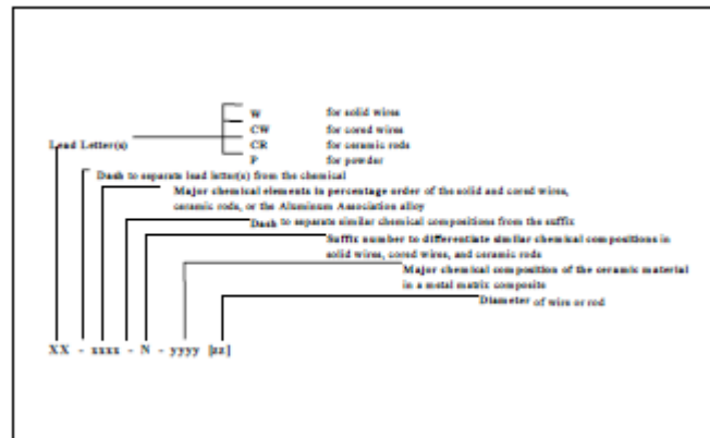
Figure 3-1. Thermal spray feedstock designation nomenclature
