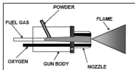
Figure 2-5. Powder gun cross section
