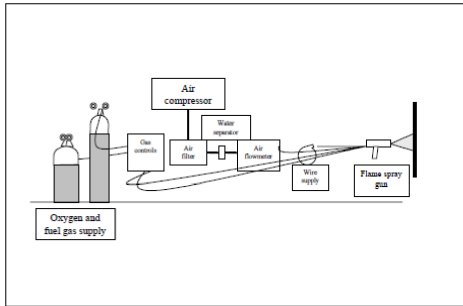
Figure 2-2. Typical flame spray system
