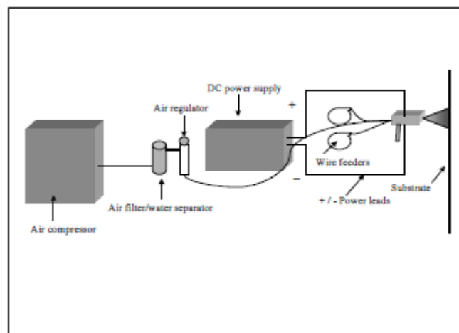
Figure 2-6. Typical two-wire arc spray system
