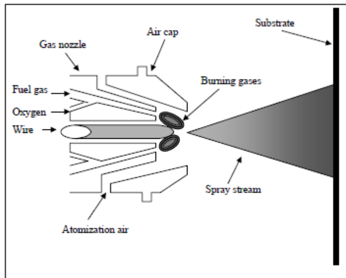
Figure 2-3. Typical flame spray gun
