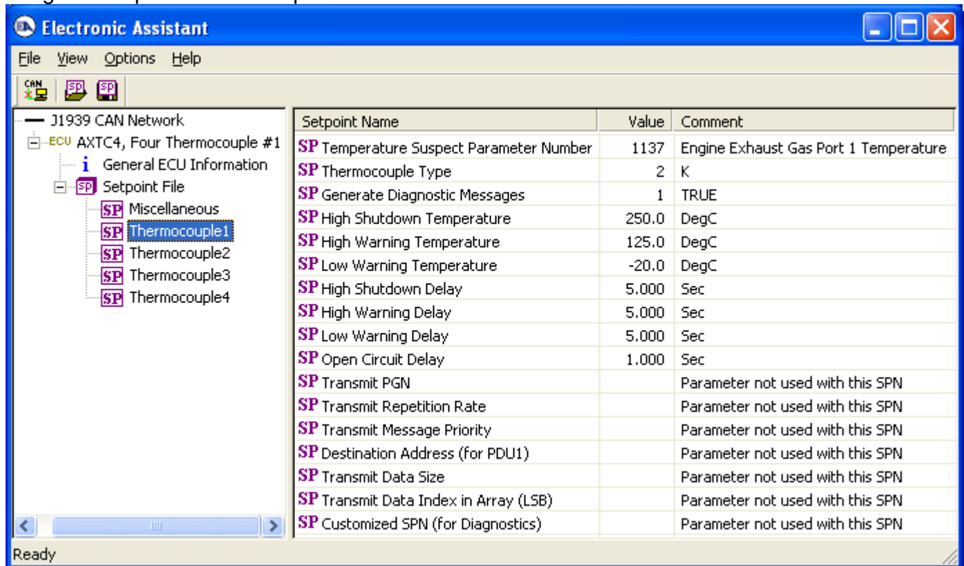
Image 5.4: Input Channel Setpoints – Defaults for Channel 1
