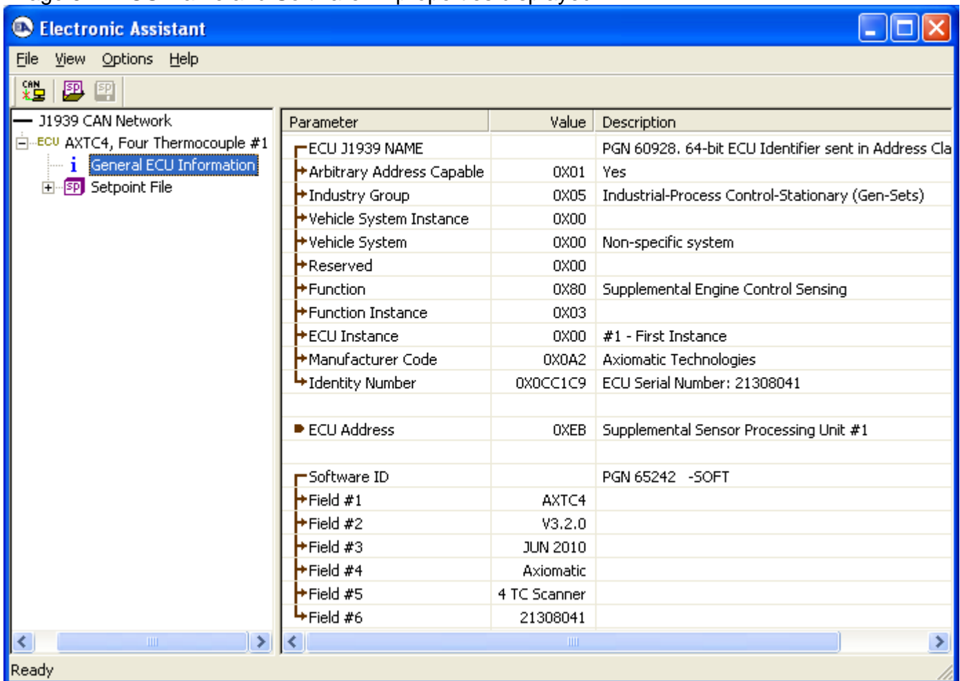
Image 5.2: ECU Name and Software ID properties displayed
