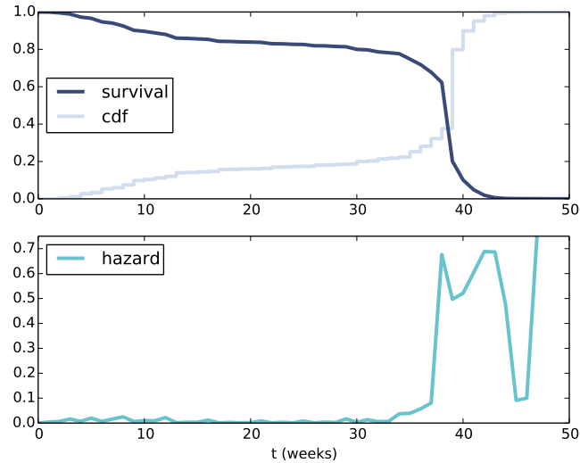
Figure 13.1: Cdf and survival curve for pregnancy length (top), hazard curve (bottom).
