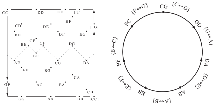
Fig. 4. ( left ) most efficient voice-leading paths between diatonic fifths form a chain that runs through the center of the Möbius strip from Figure 1. ( right ) These voice leading paths form an abstract circle, in which adjacent dyads are related by three-step diatonic transposition, and are linked by single-step voice leading.
