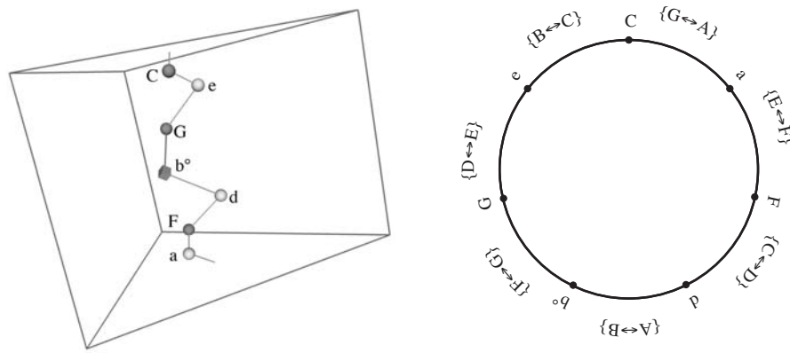
Fig. 5. ( left ) most efficient voice-leading paths between diatonic triads form a chain that runs through the center of the orbifold representing three-note chords. ( right ) These voice leading paths form an abstract circle, in which adjacent triads are linked by single-step voice leading. Note that here, adjacent triads are related by transposition by two diatonic steps.
