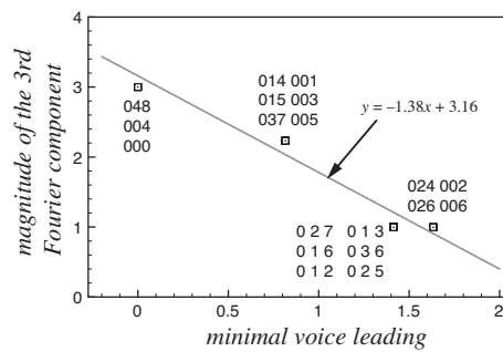
Figure 13. For trichords, the equation FC_3 = -1.38VL + 3.16 relates the third Fourier component to the Euclidean size of the minimal voice leading to the nearest subset of \{0, 4, 8\} .
