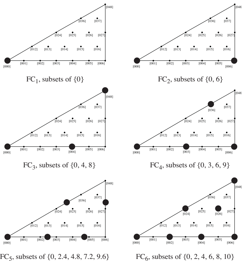
Fig. 11. The magnitude of a set class's n th Fourier component is approximately linearly related to the size of the minimal voice leading to the nearest subset of the perfectly even n -note chord, shown here as dark spheres.
