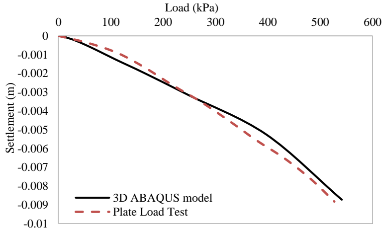
Fig. 7. Comparison of settlement result between the 3D-FE simulation and field data
