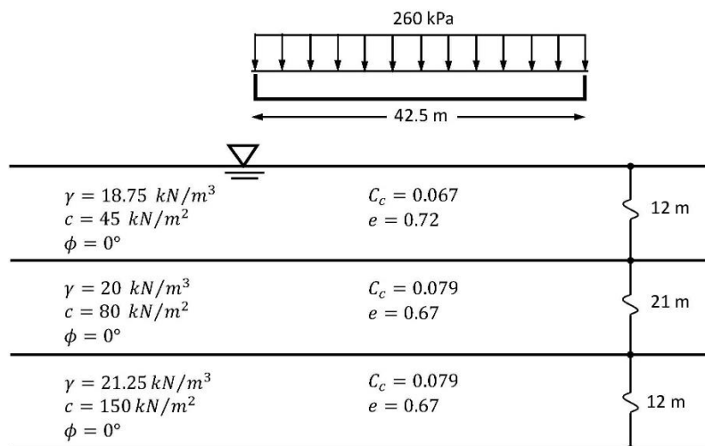
Fig. 6. Soil profile in Khayyam steel mill project in Neyshabur, Iran (in curtsey of Reinforced Earth Iran Company)
