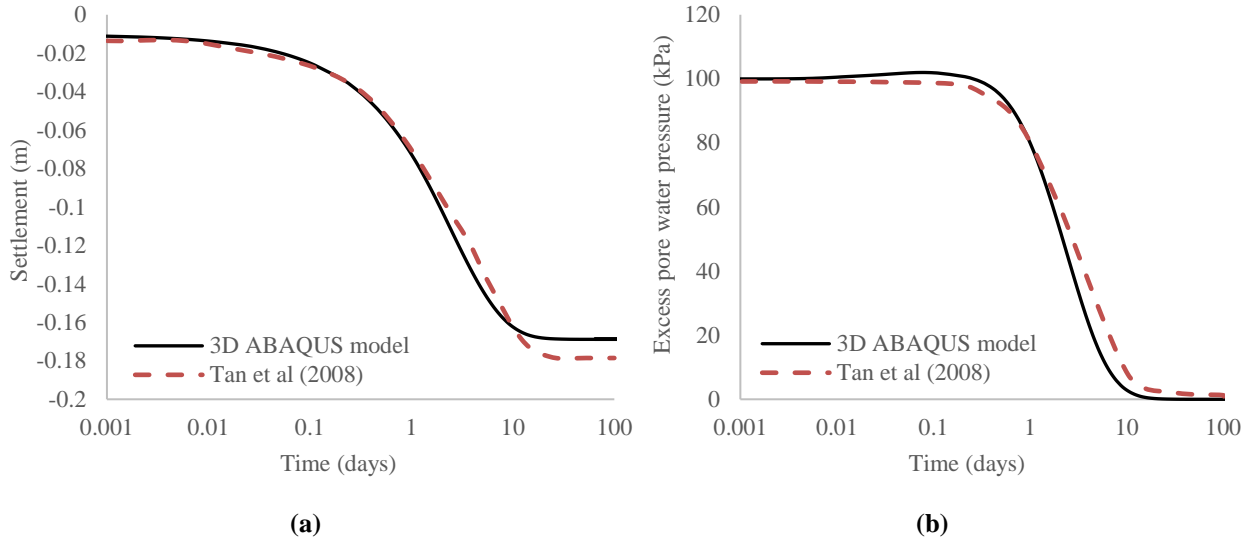
Fig. 4. 3D elastoplastic modeling: a) settlement, b) excess pore water pressure
