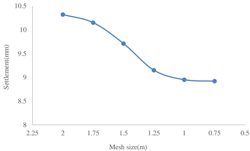
Fig. 2. Mesh convergence analysis for the FE model
