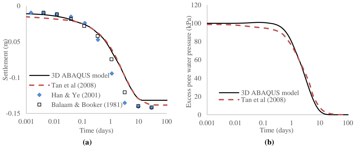
Fig. 3. 3D elastic modeling: a) settlement, b) excess pore water pressure
