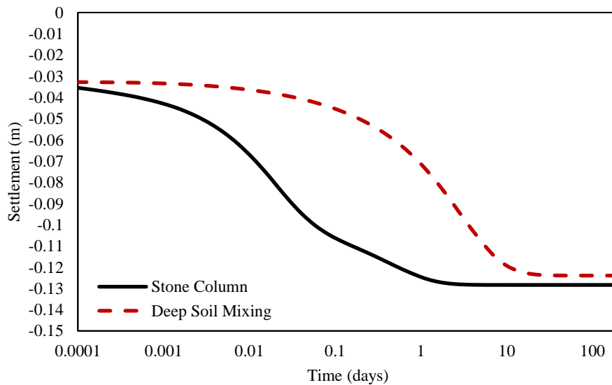
Fig. 11. Comparison the amount of settlement and the consolidation rate of stone columns to DSM columns
