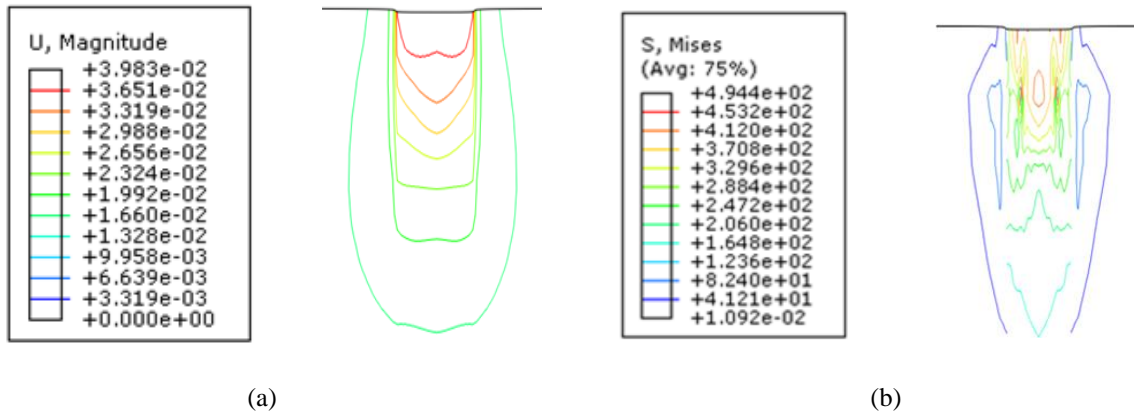
Fig. 8. Bulging of one of the stone column in group under plate loading test: a) Displacement contours (m), b) Stress contours (kPa)
