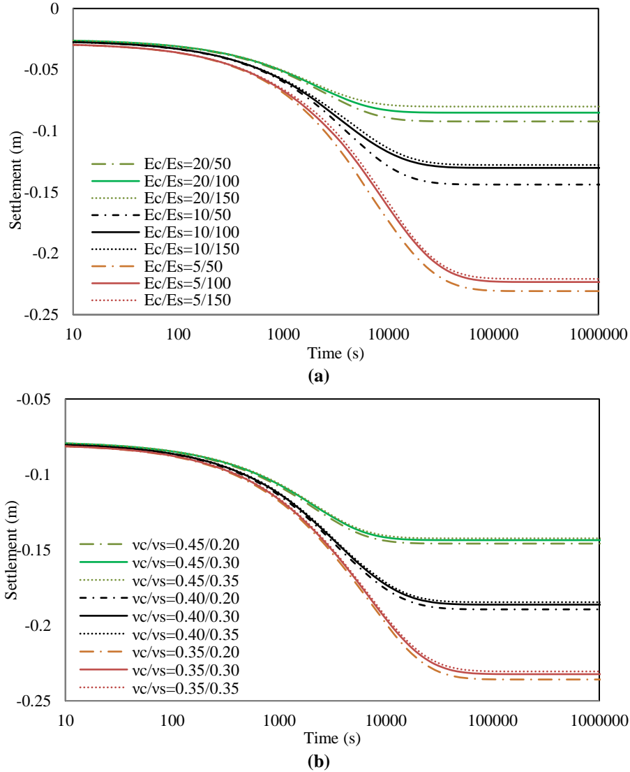
Fig. 10. Parametric studies for material properties: a) effect of elastic modulus, b) effect of Poisson's ratio
