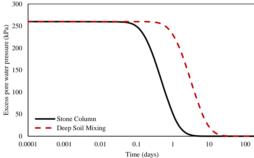
Fig. 12. Comparison the dissipation of excess pore water pressure of stone columns to DSM columns
