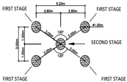
Fig. 5. Arrangement of stone columns in Khayyam Neyshabur (in curtesy of Reinforced earth Iran Company)
