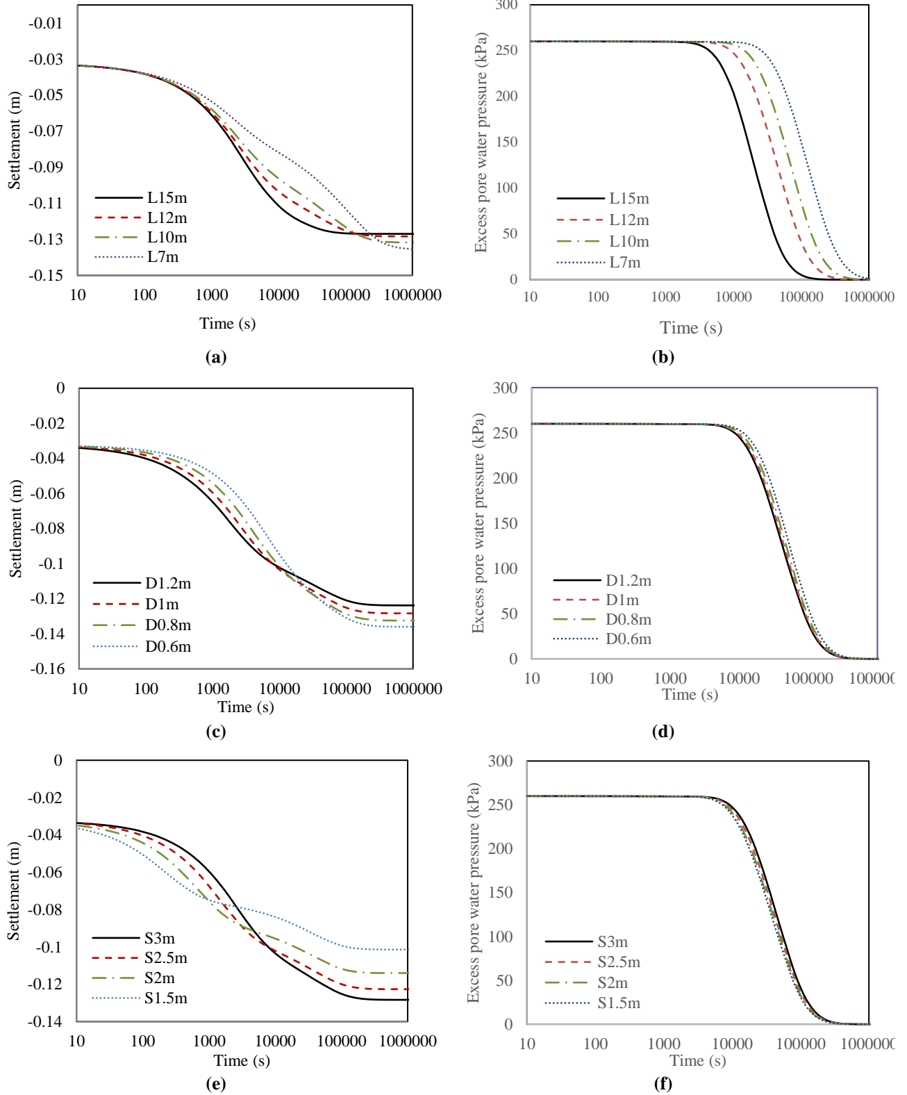
Fig. 9. Parametric studies for geometric characteristics: a) and b) The effect of length of column, c) and d) The effect of column diameter, e) and f) The effect of spacing between the stone columns
