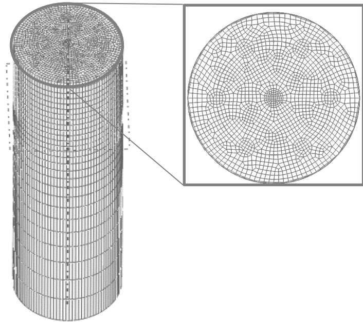
Fig. 1. Model geometry and finite element mesh
