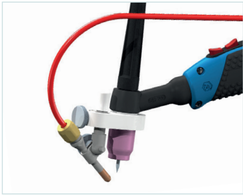
Aportador de hilo frio / TIG-Cold-Wire-Feeding
