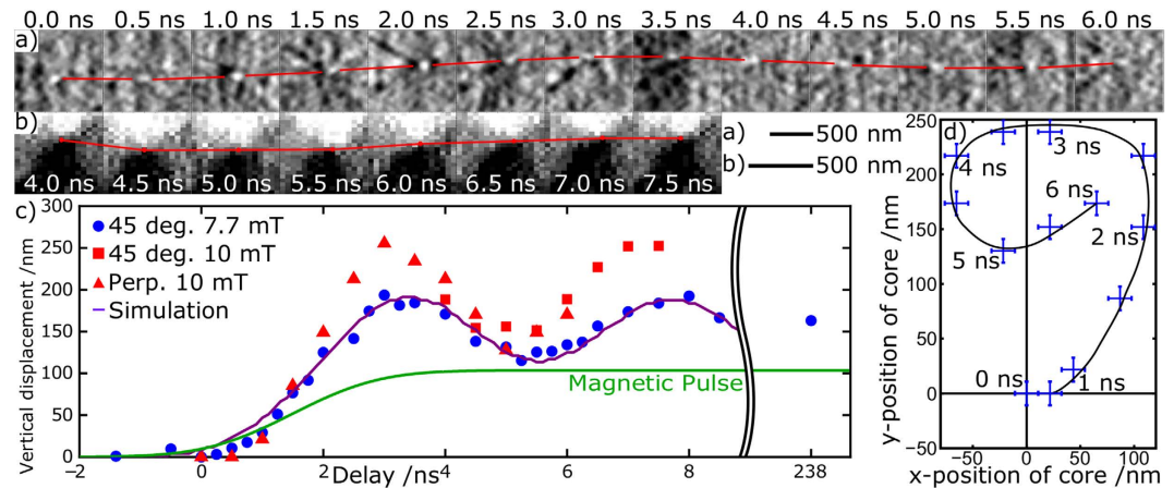
Figure 3. Vortex gyration. Close-up of the reconstructed magnetic contrast around the core taken at different values of the delay time \Delta t for (a) 90^\circ and (b) for 45^\circ ( 3.7 \text{ V} pulse) angle-of-incidence. The lines trace the vortex core position. (c) The vertical displacement of the vortex core at different delay times. The purple line shows vertical displacement extracted from micromagnetic simulations. The simulated magnetic pulse profile is shown by the green line. The point at 238 \text{ ns} delay gives the vertical position of the core after being fully damped. The pulse length for this particular point was increased to 500 \text{ ns} to allow verifying the vertical position of the core in this case. (d) The position of the vortex core in the xy plane at various delay times imaged in perpendicular orientation.
