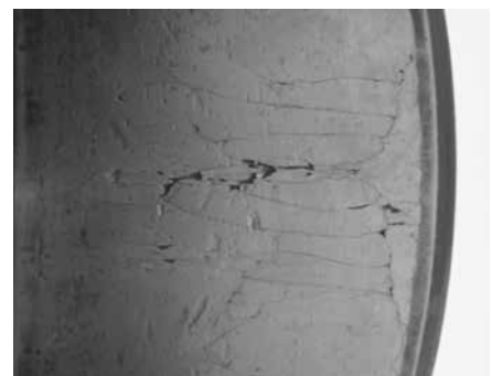
This cylindrical roller bearing inner ring was crushed by an application failure during service.
