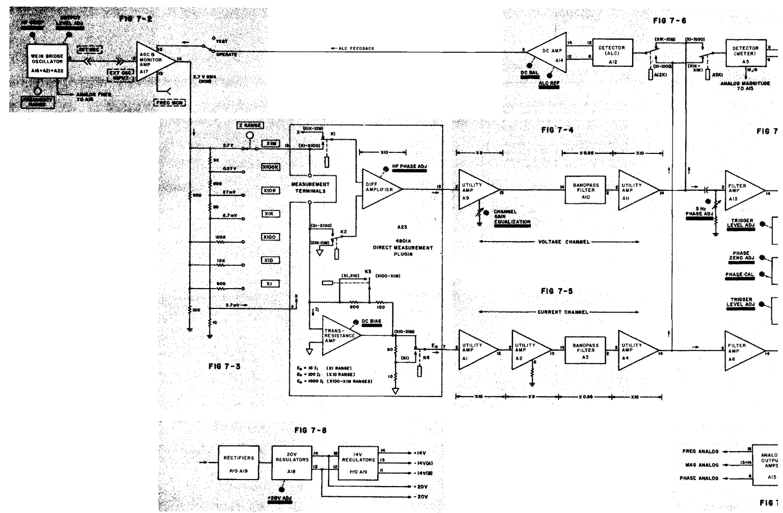
Figure 7-1. FUNCTIONAL BLOCK DIAGRAM
