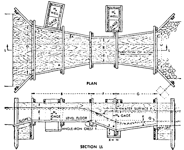
Figure F-11. Plan and elevation of the Parshall measuring flume.
