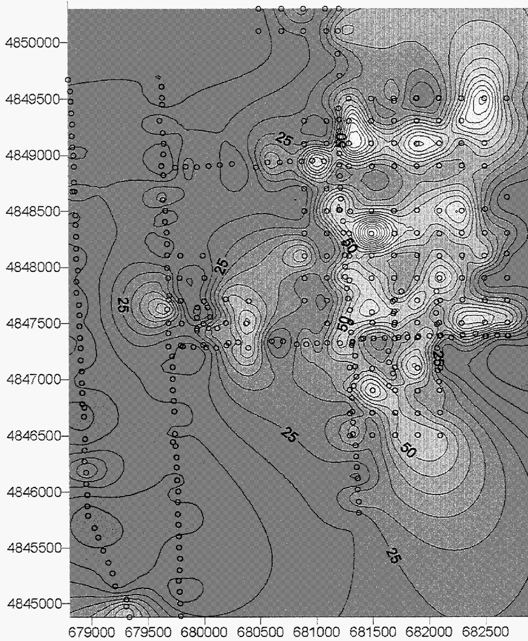
FIGURE 9. Contour map of microbial data collected over Vernon Field, summer 2000.
