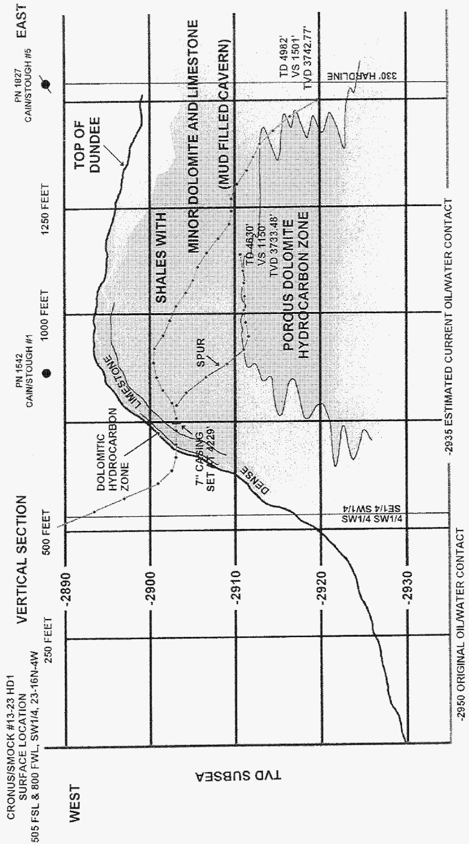
VERNON FIELD ST. VERNON & SMOCK #13-23 HD1 WELLBORE SCHEMATIC
