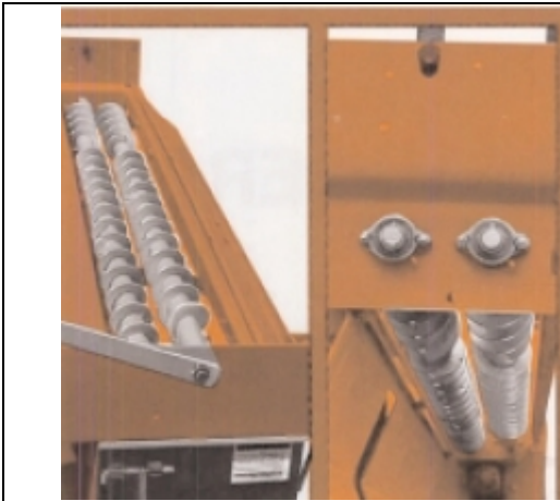
Figure 15: Auger Image
