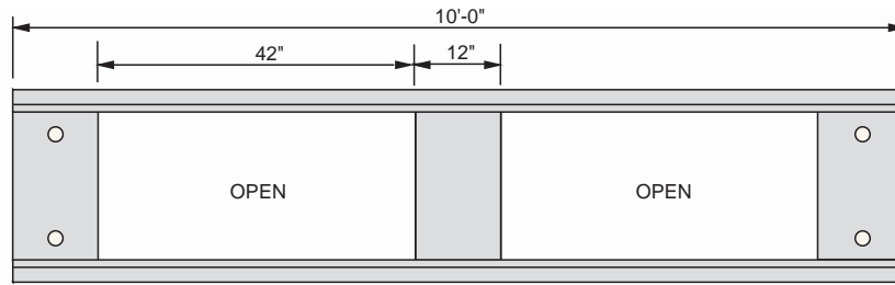
PLAN VIEW
