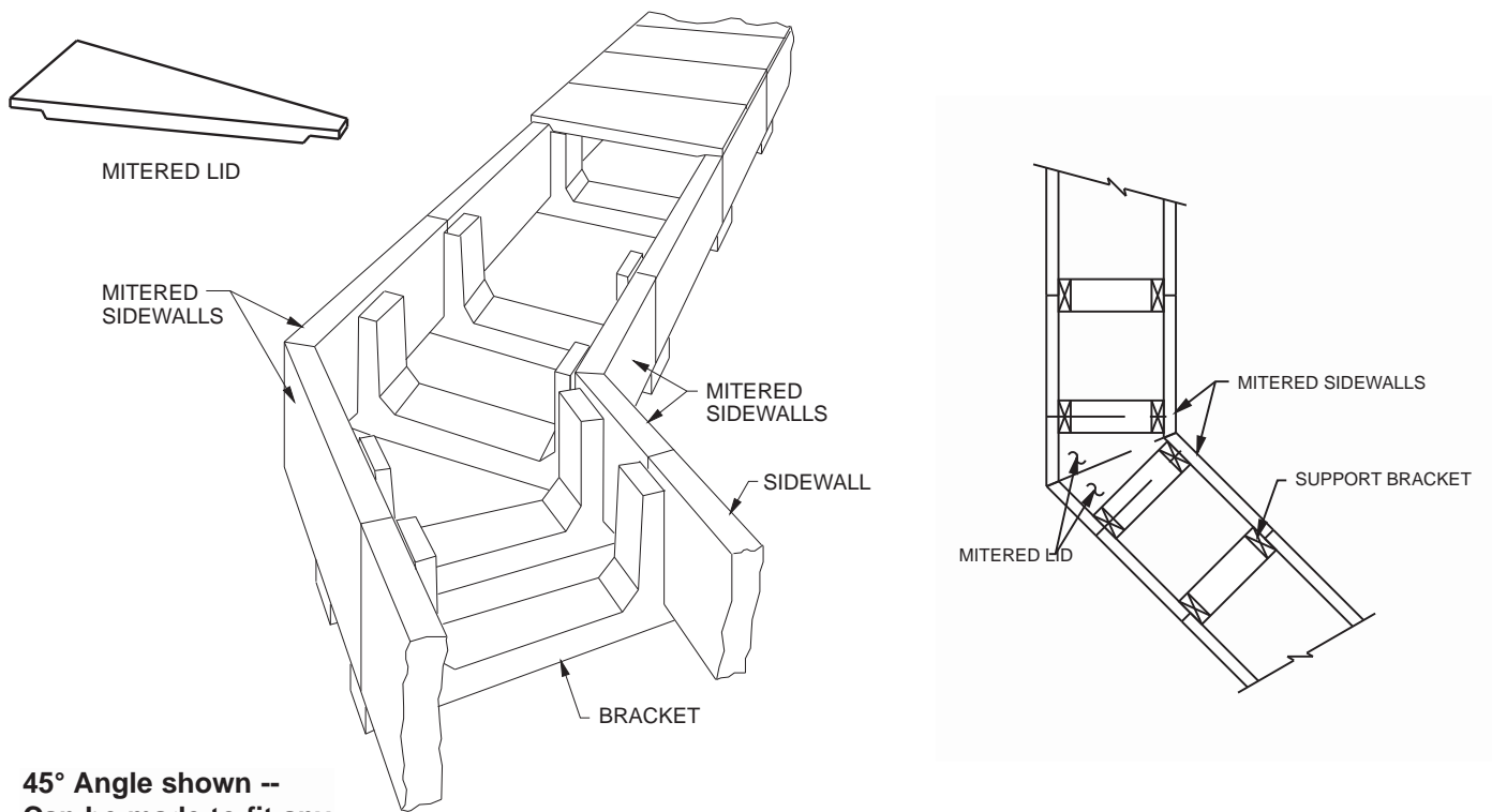
Mitered turn
