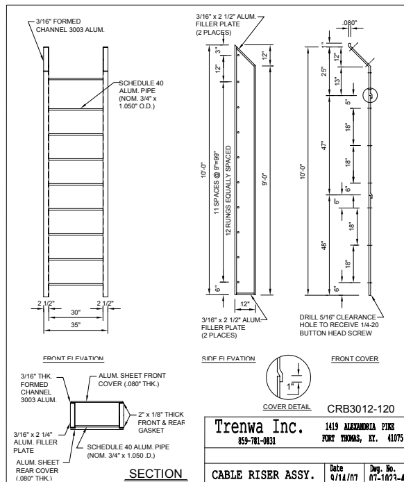
EXAMPLE DRAWING
