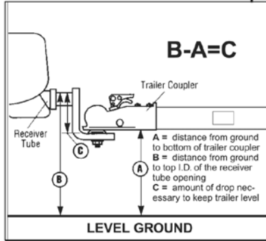
To Measure Ball Mount Drop:
