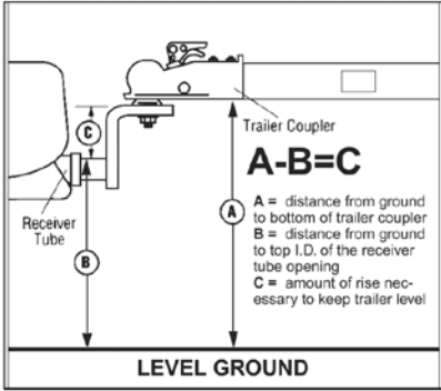
To Measure Ball Mount Rise:
