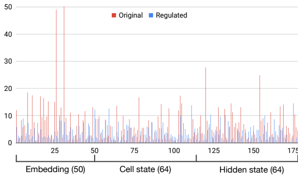
Figure 10: An example of vector d for an LSTM model.
