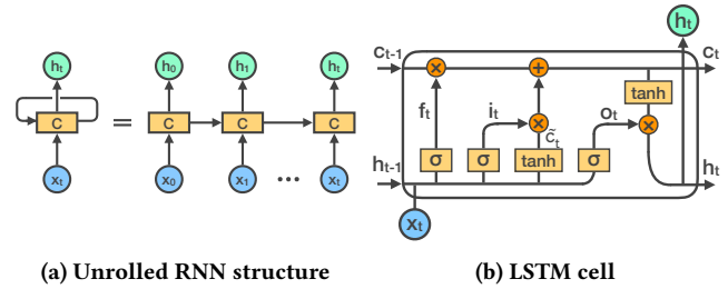
Figure 1: Architecture of recurrent neural networks. (a) An unrolled representation of RNN architecture. (b) The internal structure of Long Short Term Memory networks.
