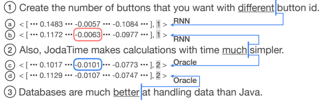
Figure 5: Analysis of an example text (shown in ②). Vectors Ⓐ-Ⓓ denote the model states (i.e., [x_t, c_{t-1}, h_{t-1}] ) at the step of the underlined words in sentences ①-③, followed by the prediction result at the end (gray background), 1 for neutral and 2 for positive. Ⓐ and Ⓑ are states generated by a buggy RNN model. Ⓒ and Ⓓ are states from the oracle. Ⓐ is a state closest to Ⓑ produced by a buggy RNN model, whereas Ⓓ is a state closest to Ⓒ by the oracle. ② is a test sentence; ① is from the training set and ③ from the validation set.
