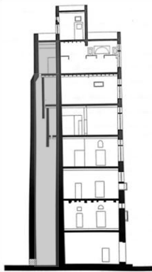
Fig.8: A section in the building where the drainage area is located. Source: Authors.
