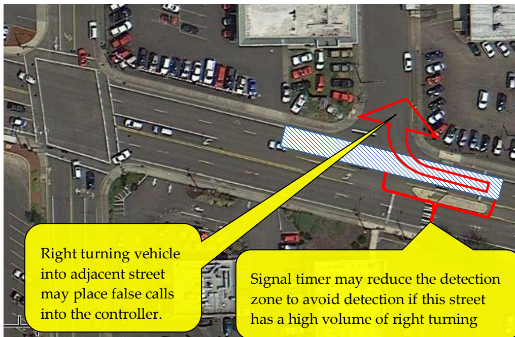
Figure 6-7 | Detection Placement Considerations: Right Turns Impacting Mainline Detection
