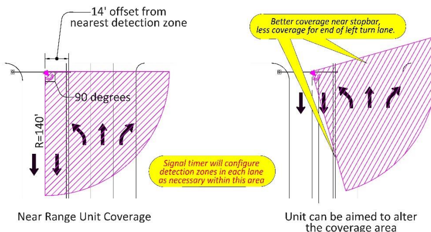
Figure 6-13 | Near Range Unit Coverage Area
