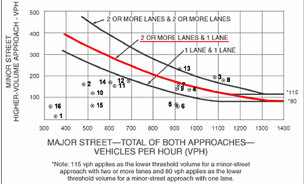
Figure 5. Example of Warrant 2, Four-Hour Vehicular Volume
