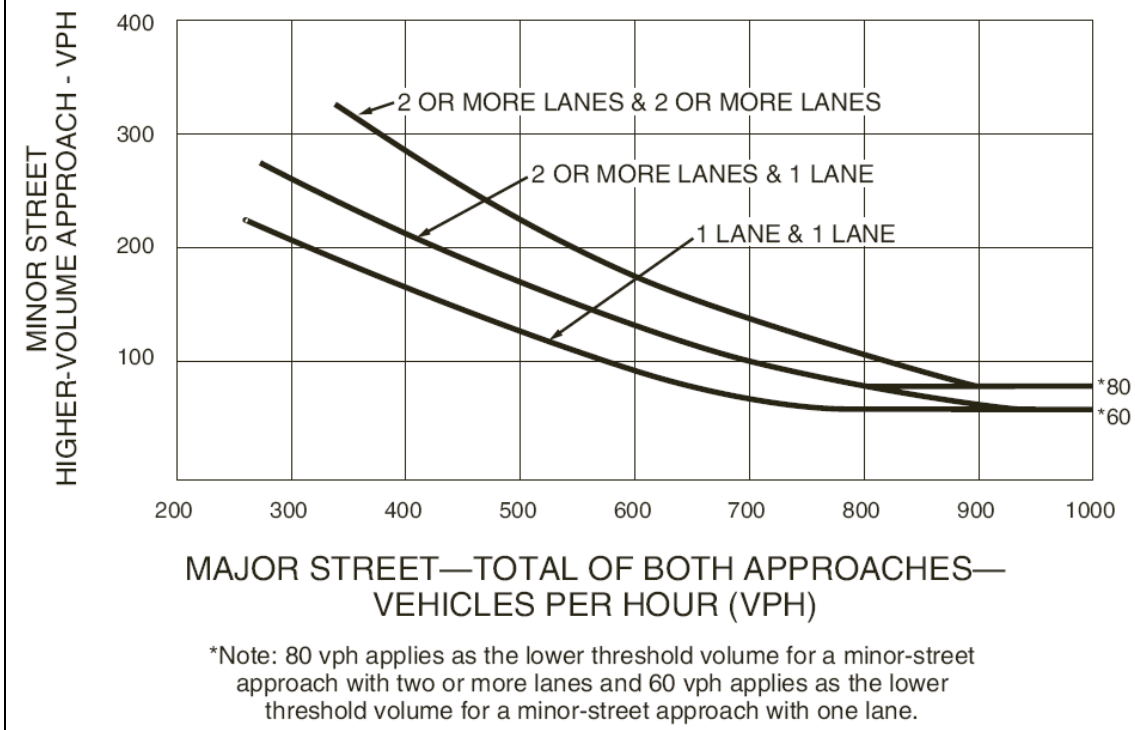
Figure 4C-2. Warrant 2, Four-Hour Vehicular Volume (70% Factor) (COMMUNITY LESS THAN 10,000 POPULATION OR ABOVE 40 mph ON MAJOR STREET)
