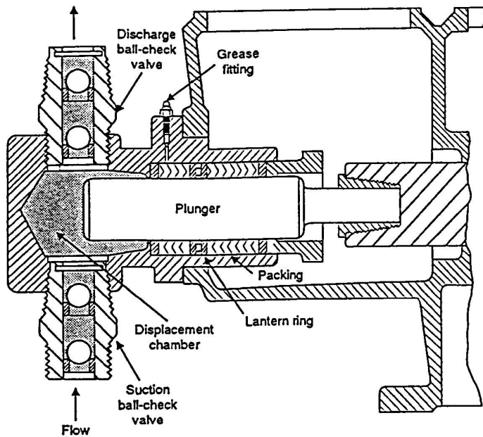
Figure 1. Cross-section drawing of the pump mechanism for a piston type chemical injection pump (Poynton, 1983).
