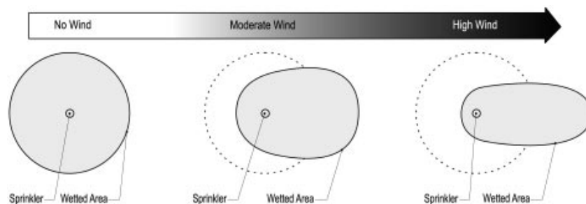
Wind impact on low pressure spray head on 5' drops
