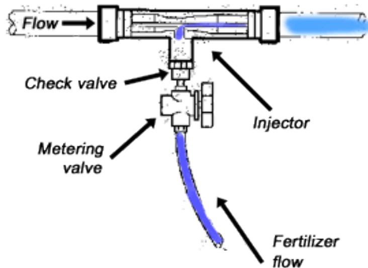
Figure 3. Schematic drawing of a venturi injector.
